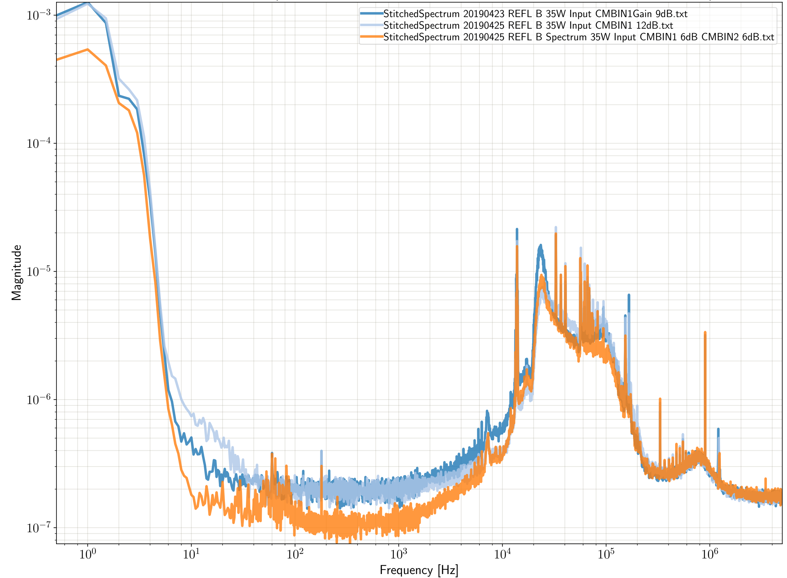
REFL B Spectra for Three CARM Configs (Out of loop +9 dB, Out of loop +12dB, and Split Sensor REFL A and B +12dB) - Apr-25-2019
