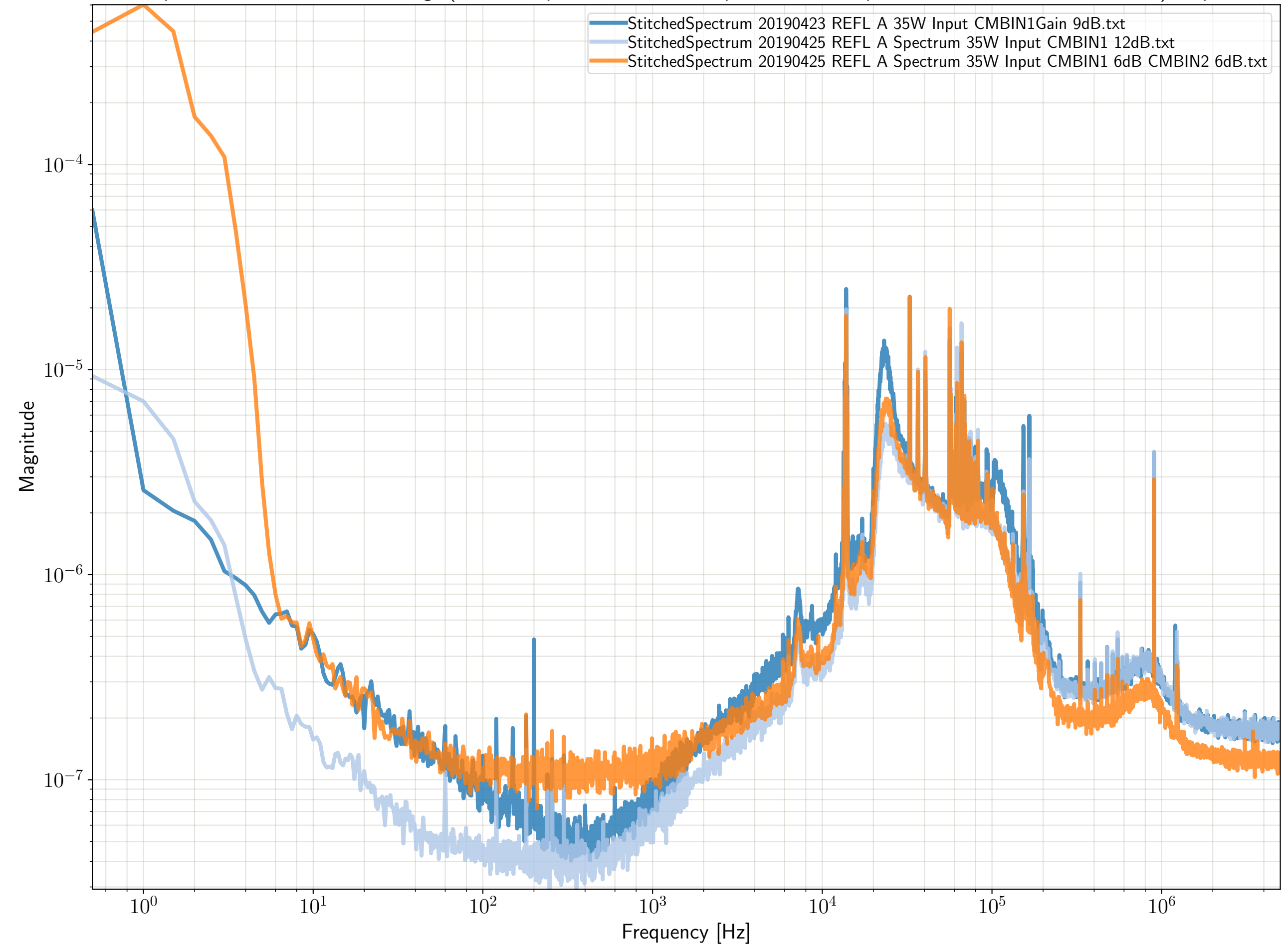
REFL A Spectra for Three CARM Configs (Out of loop +9 dB, Out of loop +12dB, and Split Sensor REFL A and B +12dB) - Apr-25-2019
