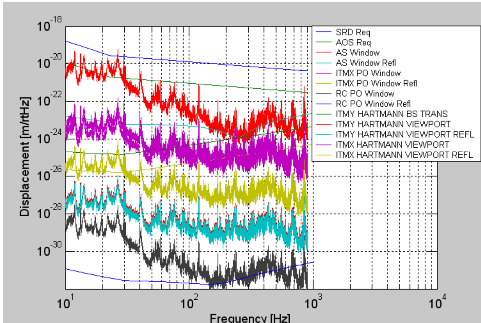
Figure 40: Output Window Scattered Light Displacement noise
