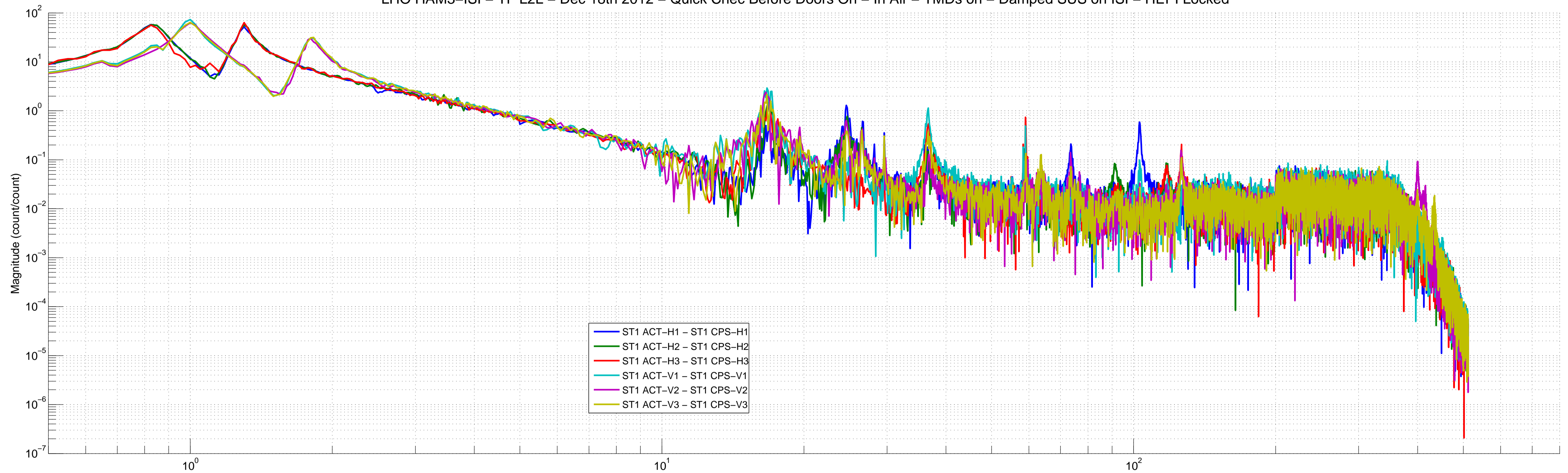
LHO HAM3-ISI - TF L2L - Dec 18th 2012 - Quick Chec Before Doors On - In Air - TMDs on - Damped SUS on ISI - HEPI Locked
