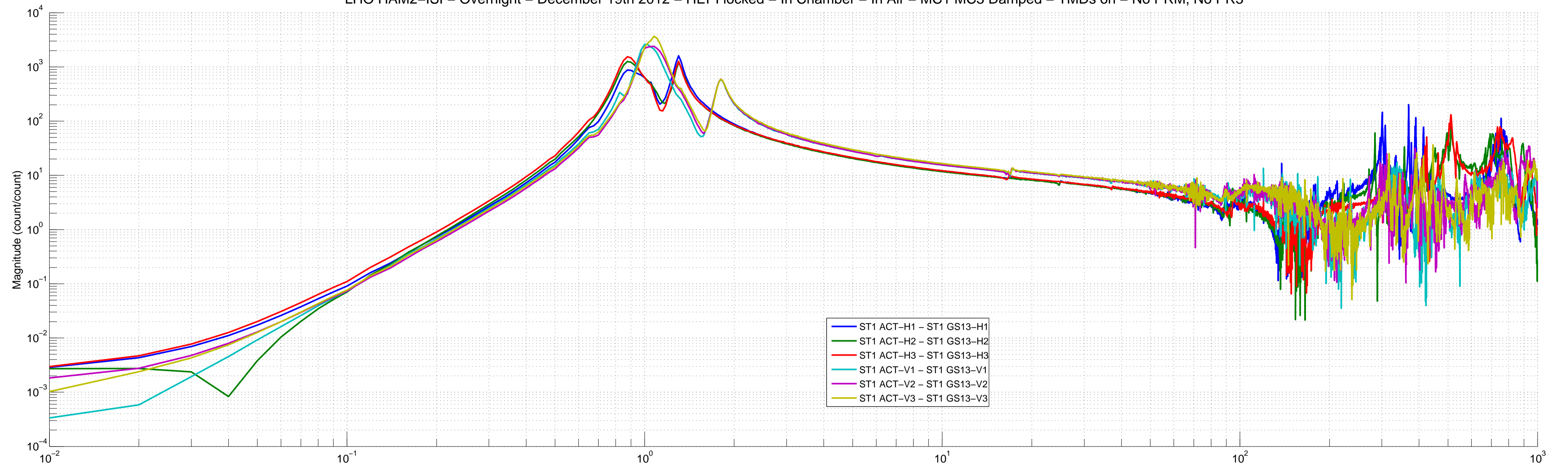
LHO HAM2-ISI – Overnight – December 19th 2012 – HEPI locked – In Chamber – In Air – MC1 MC3 Damped – TMDs on – No PRM, No PR3
