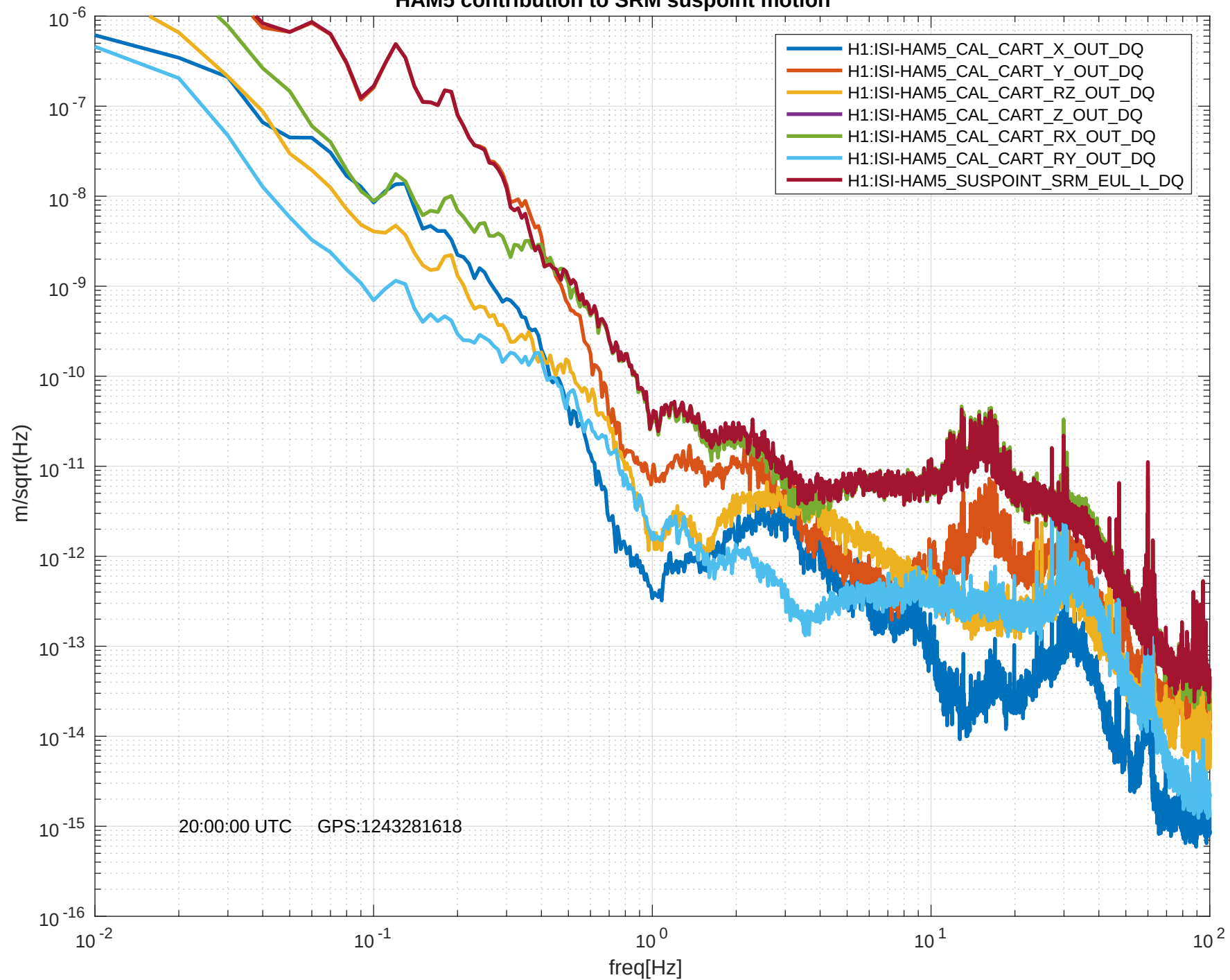
HAM5 contribution to SRM suspoint motion
