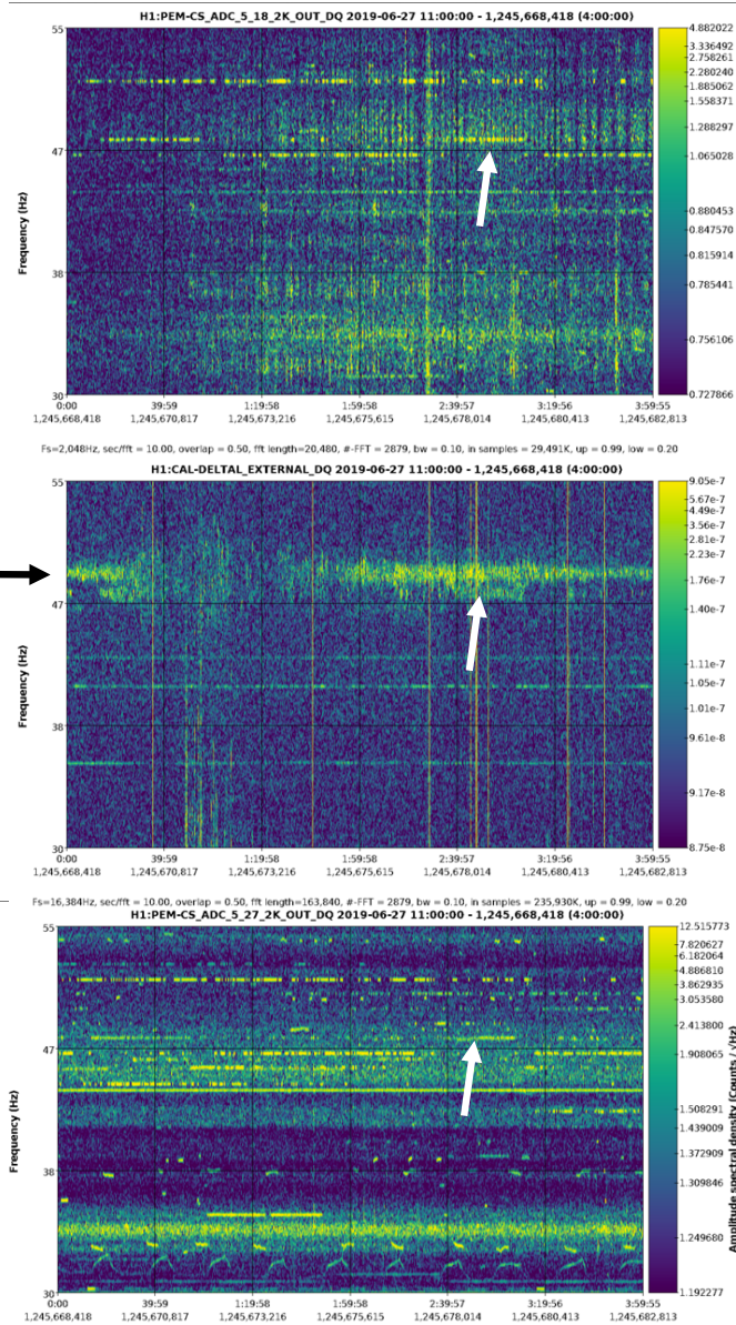
Vibrometer on strut of X-arm TCS M2 copper mirror
