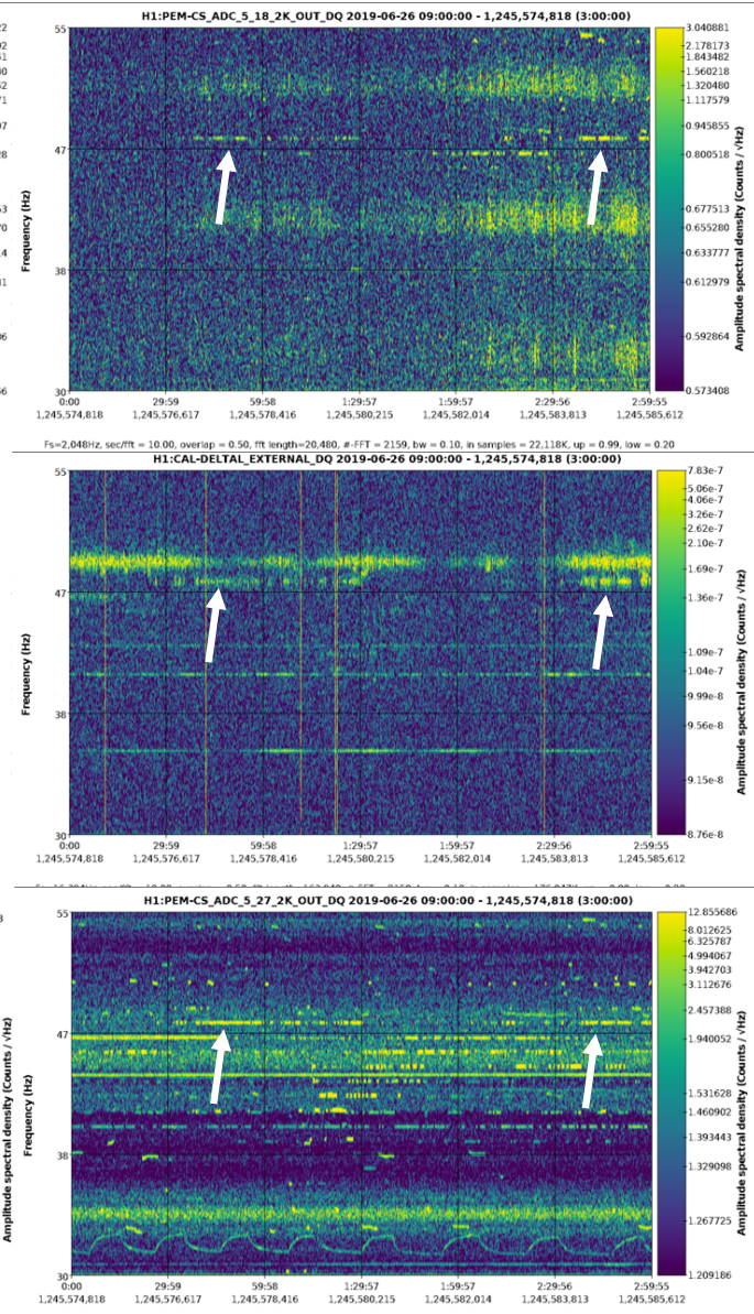
Vibrometer on strut of Y-arm TCS M2
