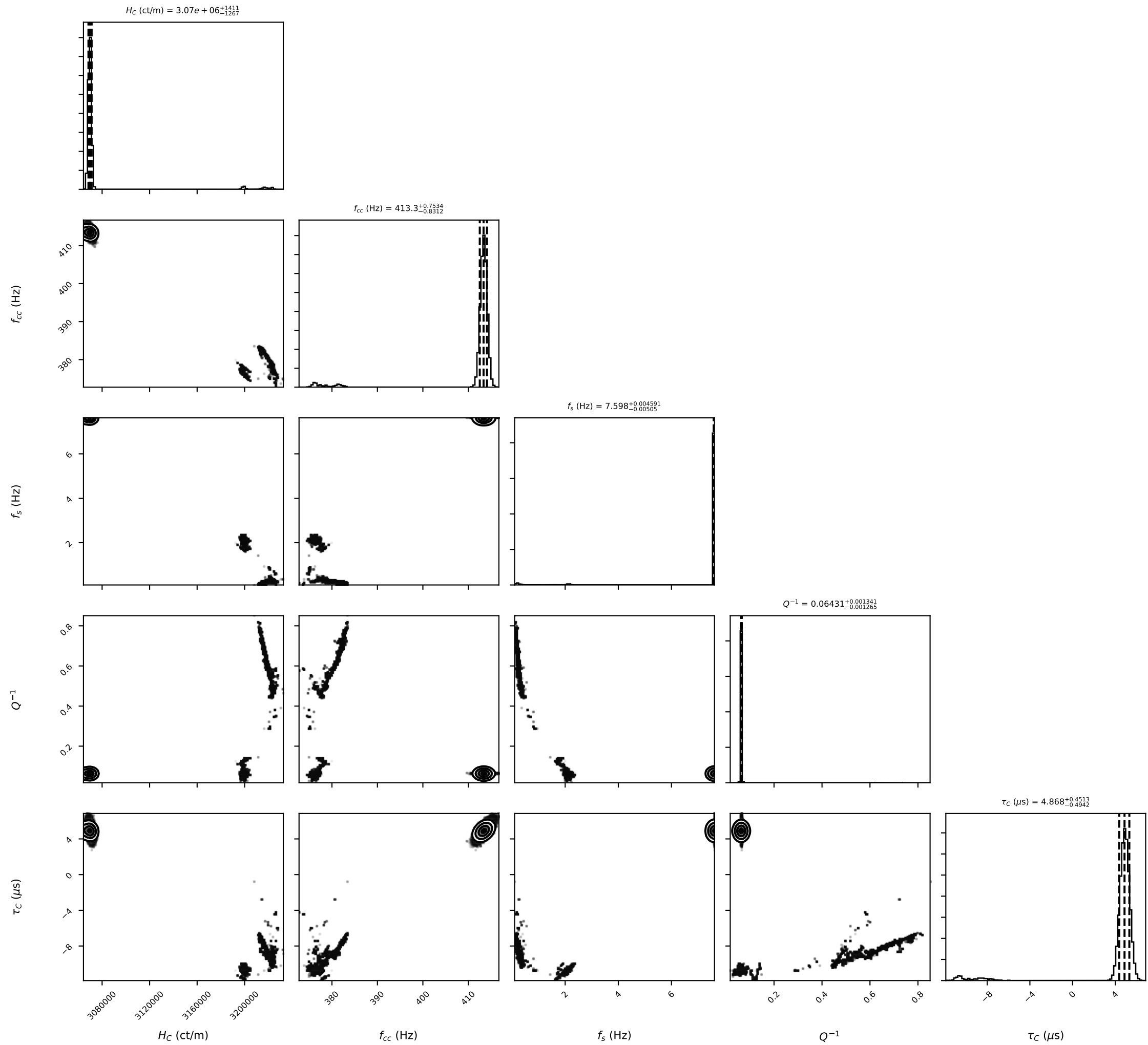
2019-08-08 H1 Sensing Function: MCMC Corner Plot
