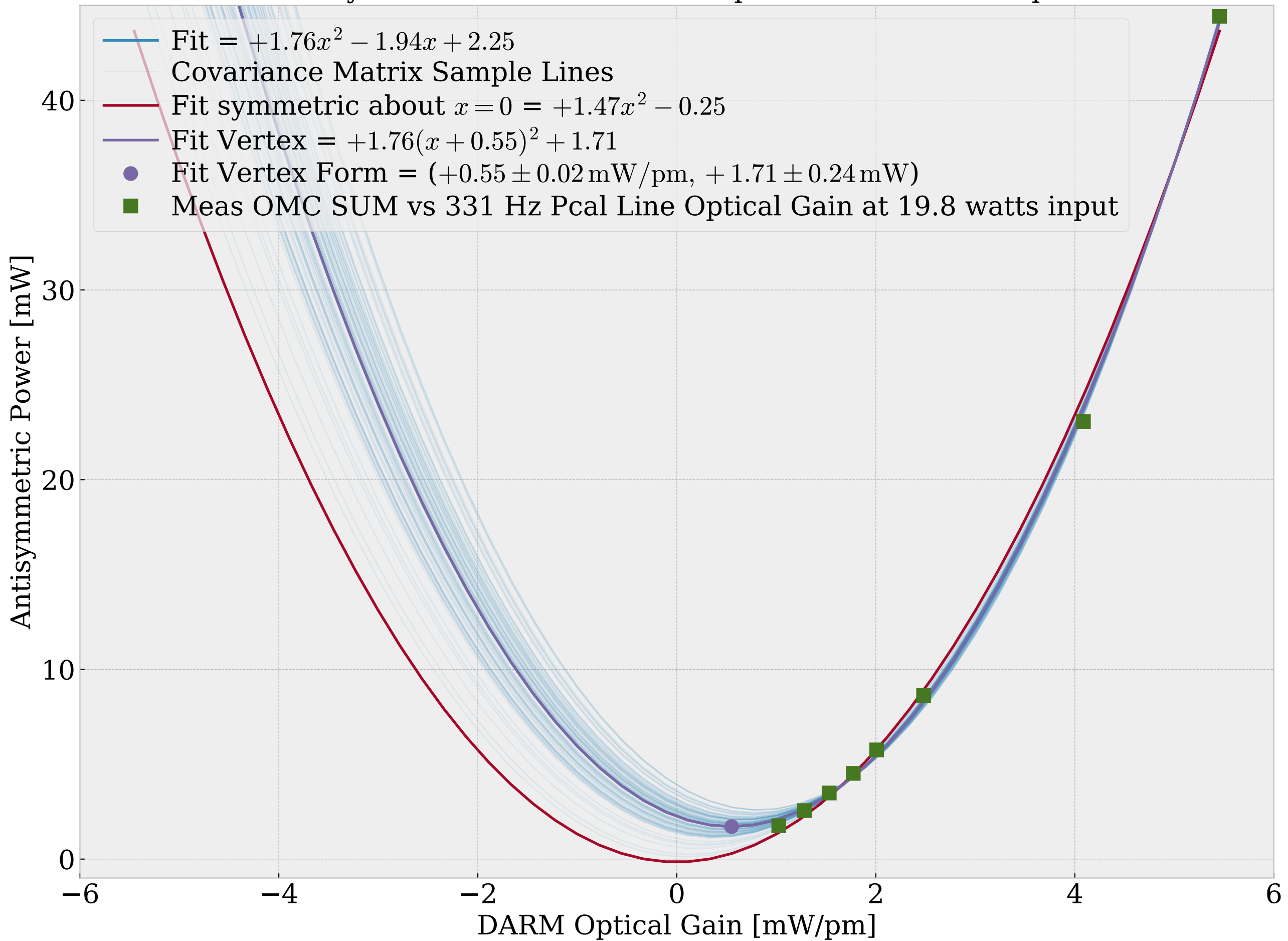
Antisymmetric Power vs DARM Optical Gain at 20 W Input
