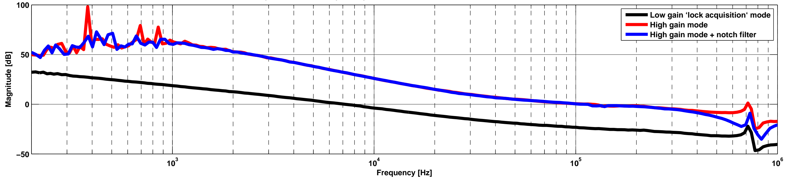
LHO Input mode cleaner open loop transfer functions measured at servo board 01/18/2013
