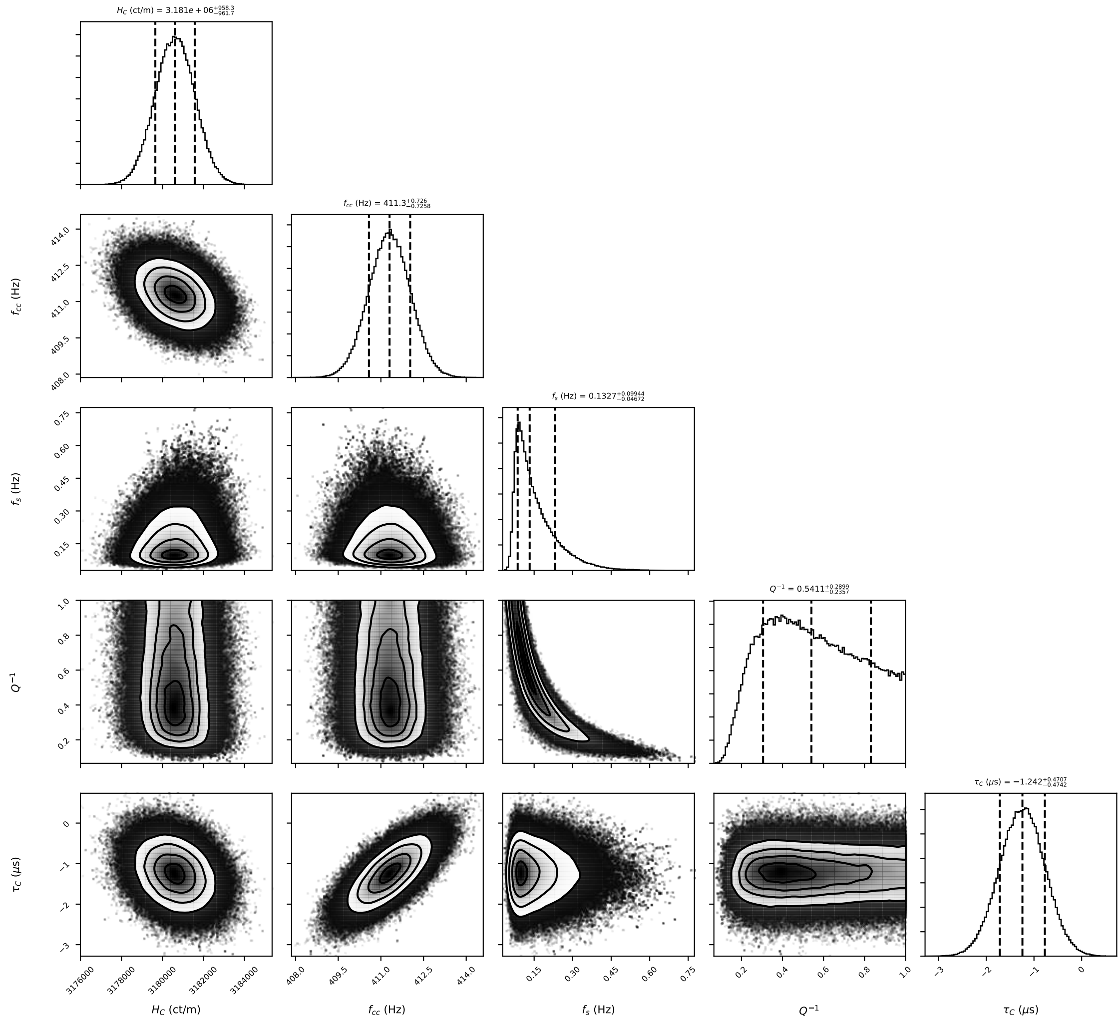
2019-09-04 H1 Sensing Function: MCMC Corner Plot
