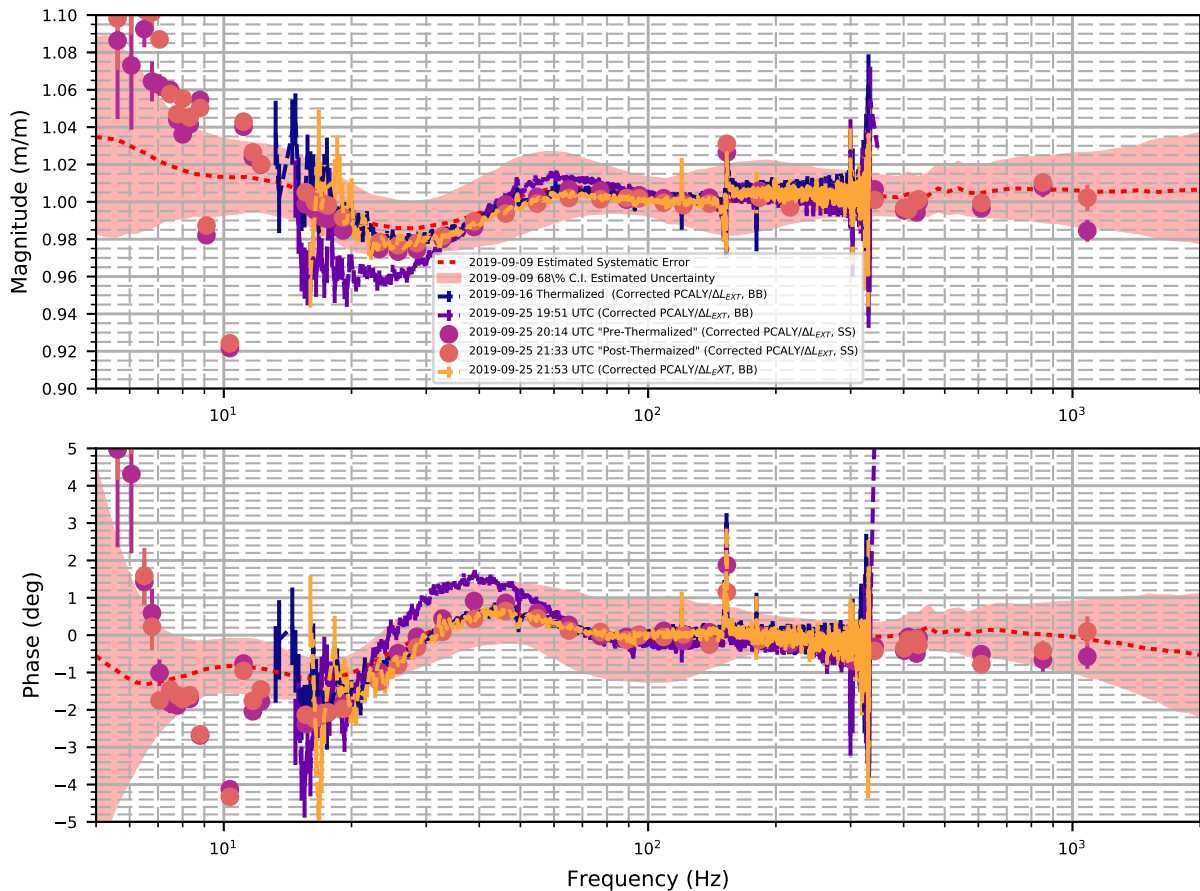
Corrected Front-end \Delta L_{EXT} DARM Displacement vs. PCALY DARM Displacement
