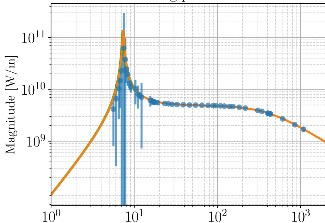
DARM sensing plant - 2019 08 19
