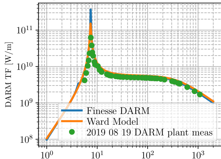
Comparison Finesse and Ward DARM Models
