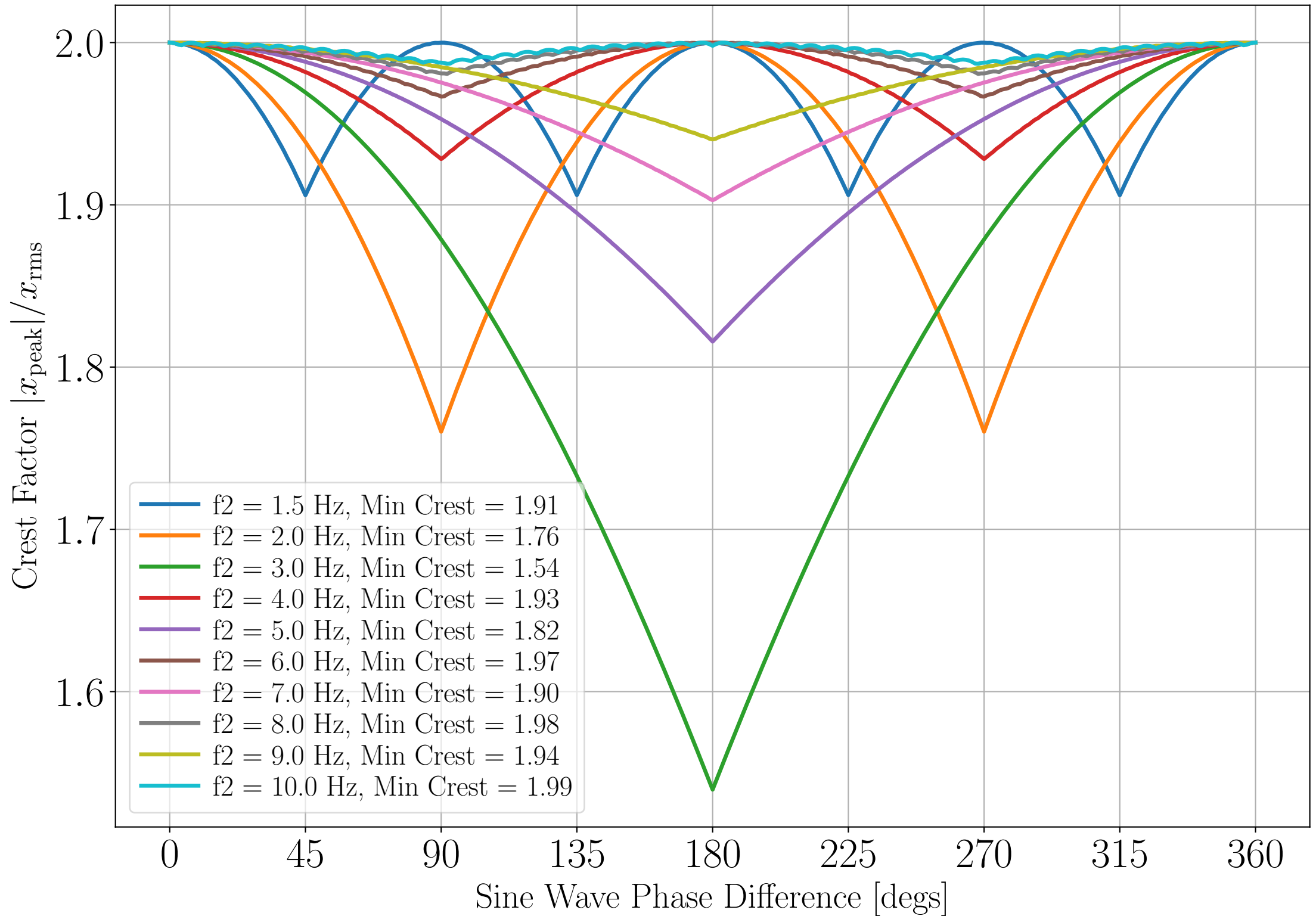
Crest Factor vs Phase Difference for Two Cosines ( f_1 = 1.0\text{Hz} )
