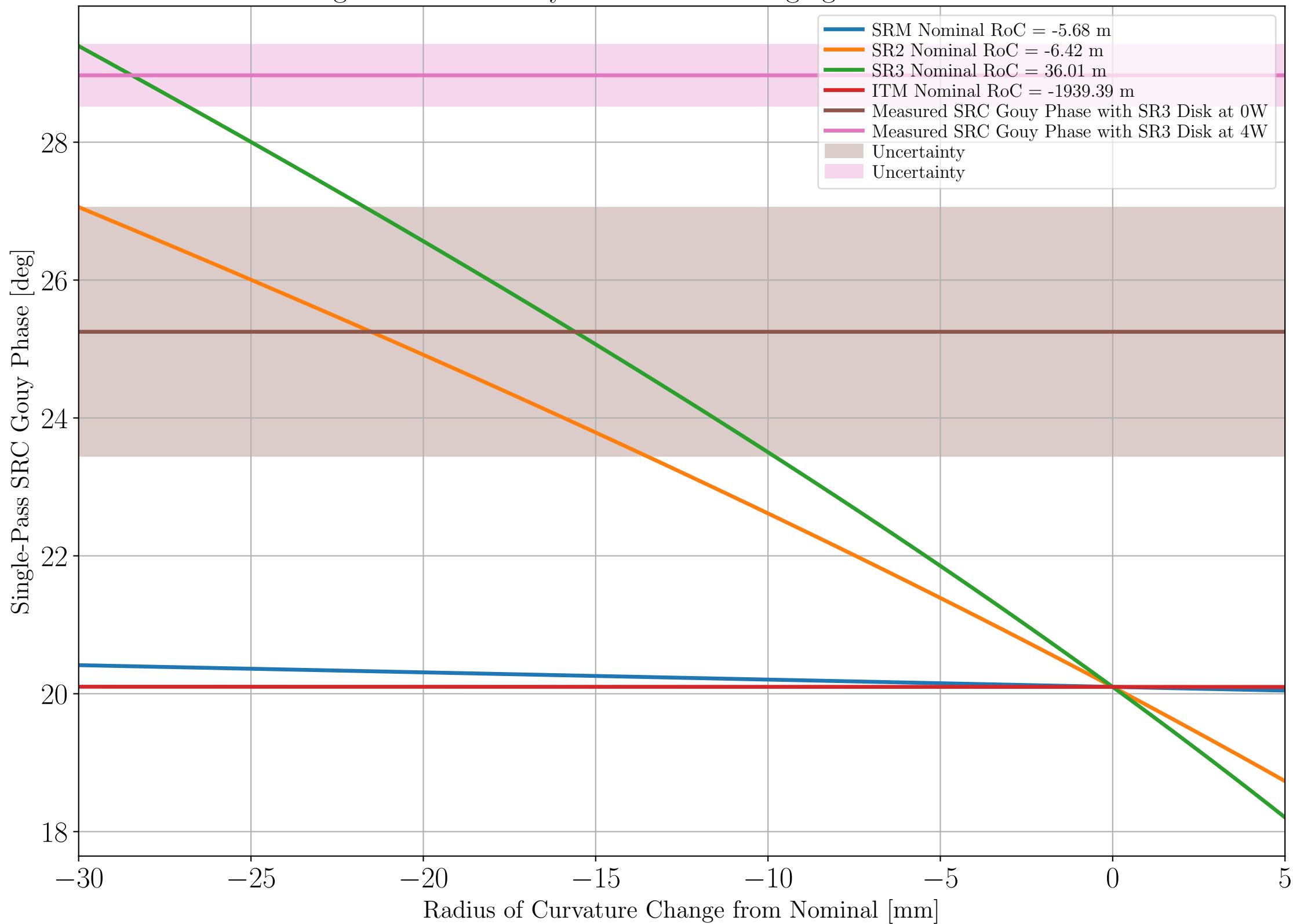
Single-Pass SRC Gouy Phase when Changing Radii of Curvature
