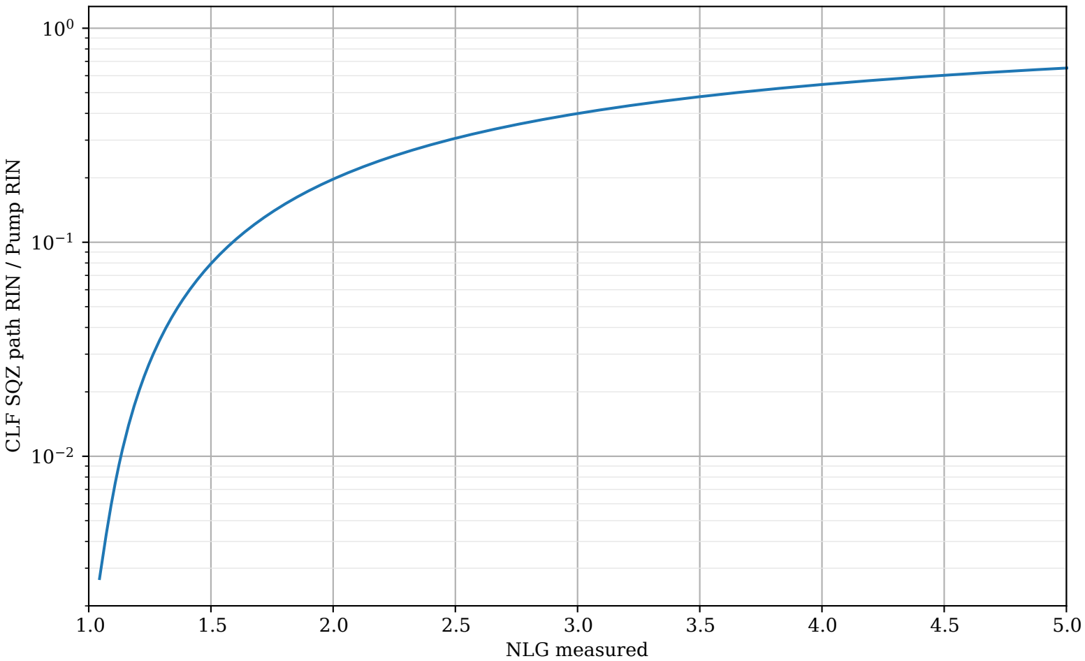
OPO parametric transfer of Pump RIN to CLF RIN
