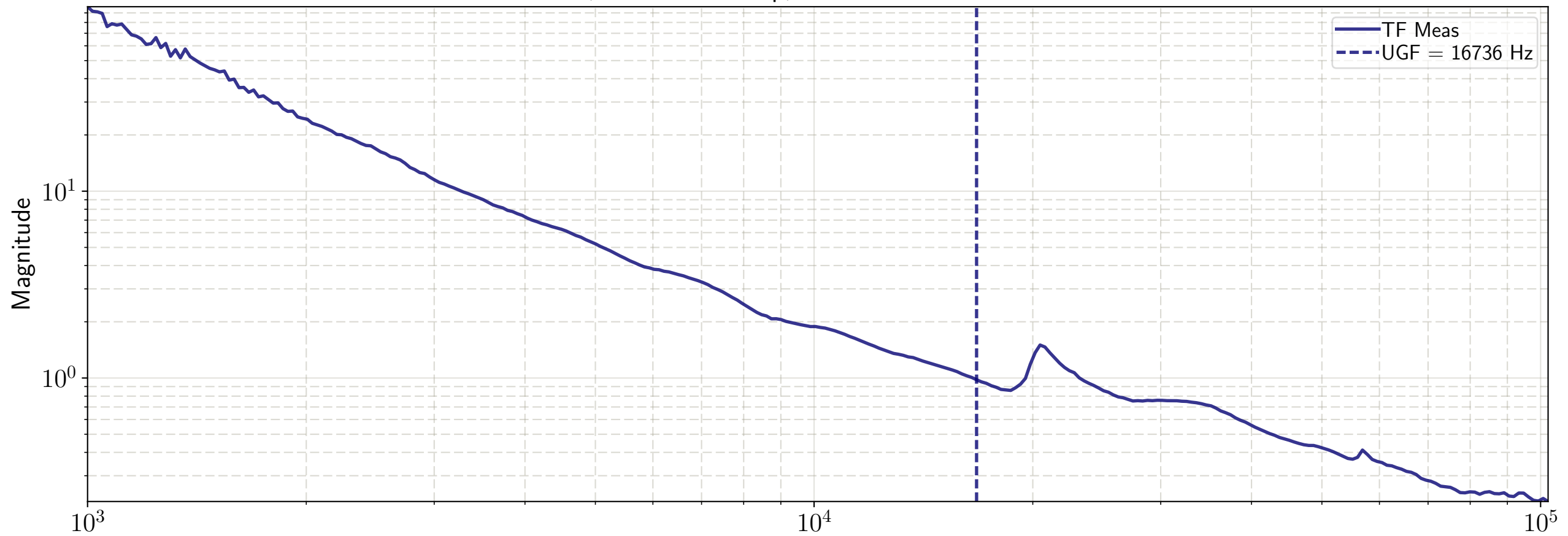
CARM OLG at 2W, Prior to Powerup, IMC IN1 moved down 2 dB - Oct-30-2019
