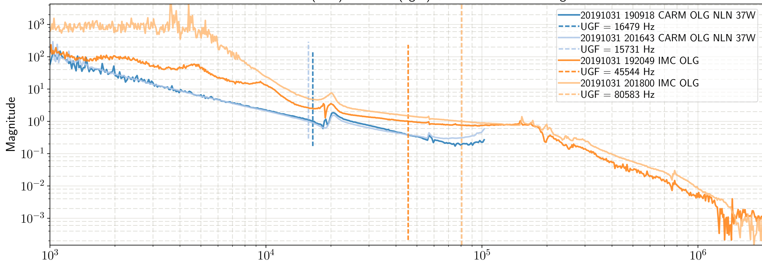
CARM and IMC OLGs before (dark) and after (light) +3dB on FSS common gain - Oct-31-2019
