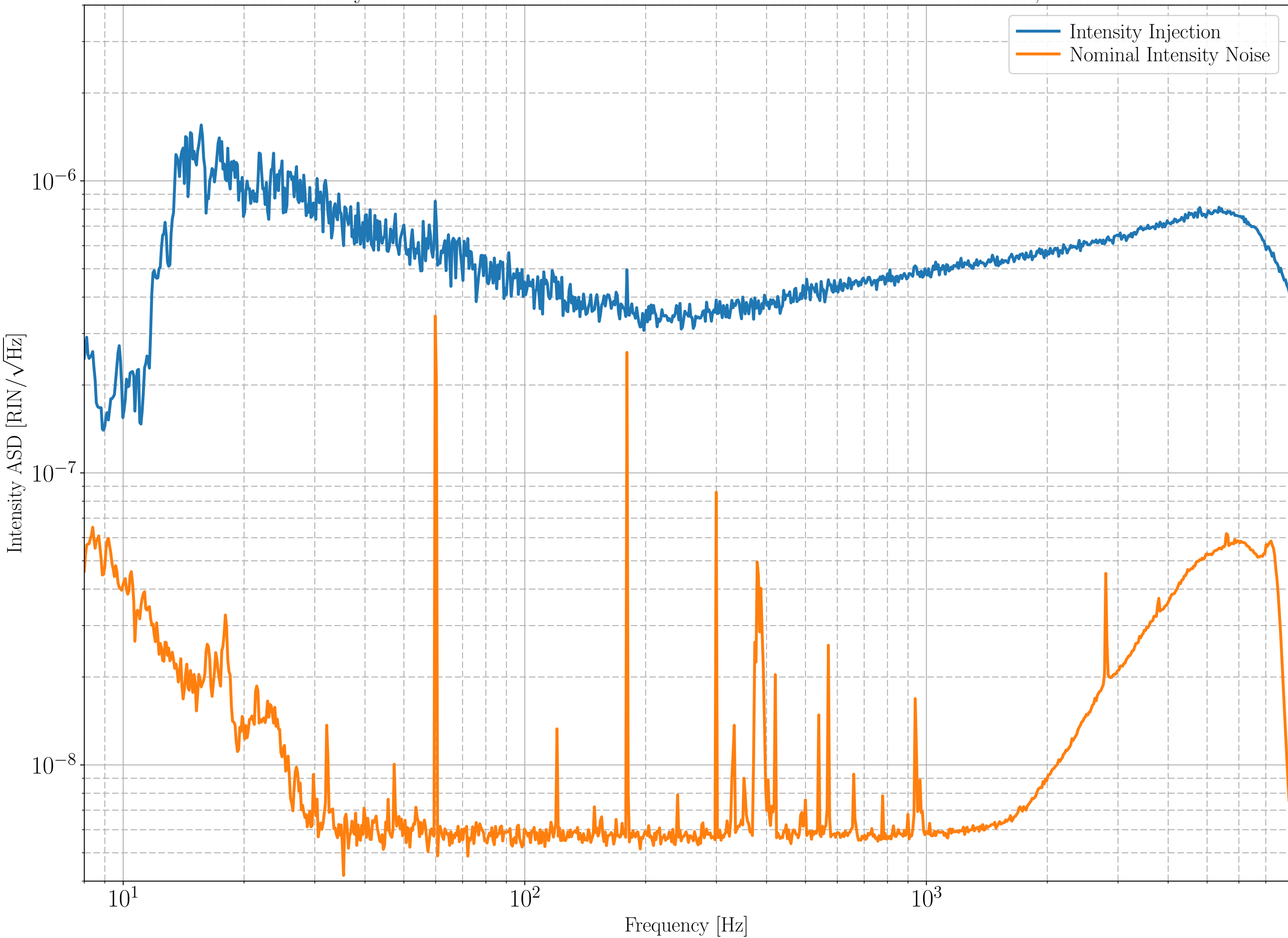
Intensity Noise - H1:PSL-ISS SECONDLOOP RIN OUTER OUT - Nov 01, 2019
