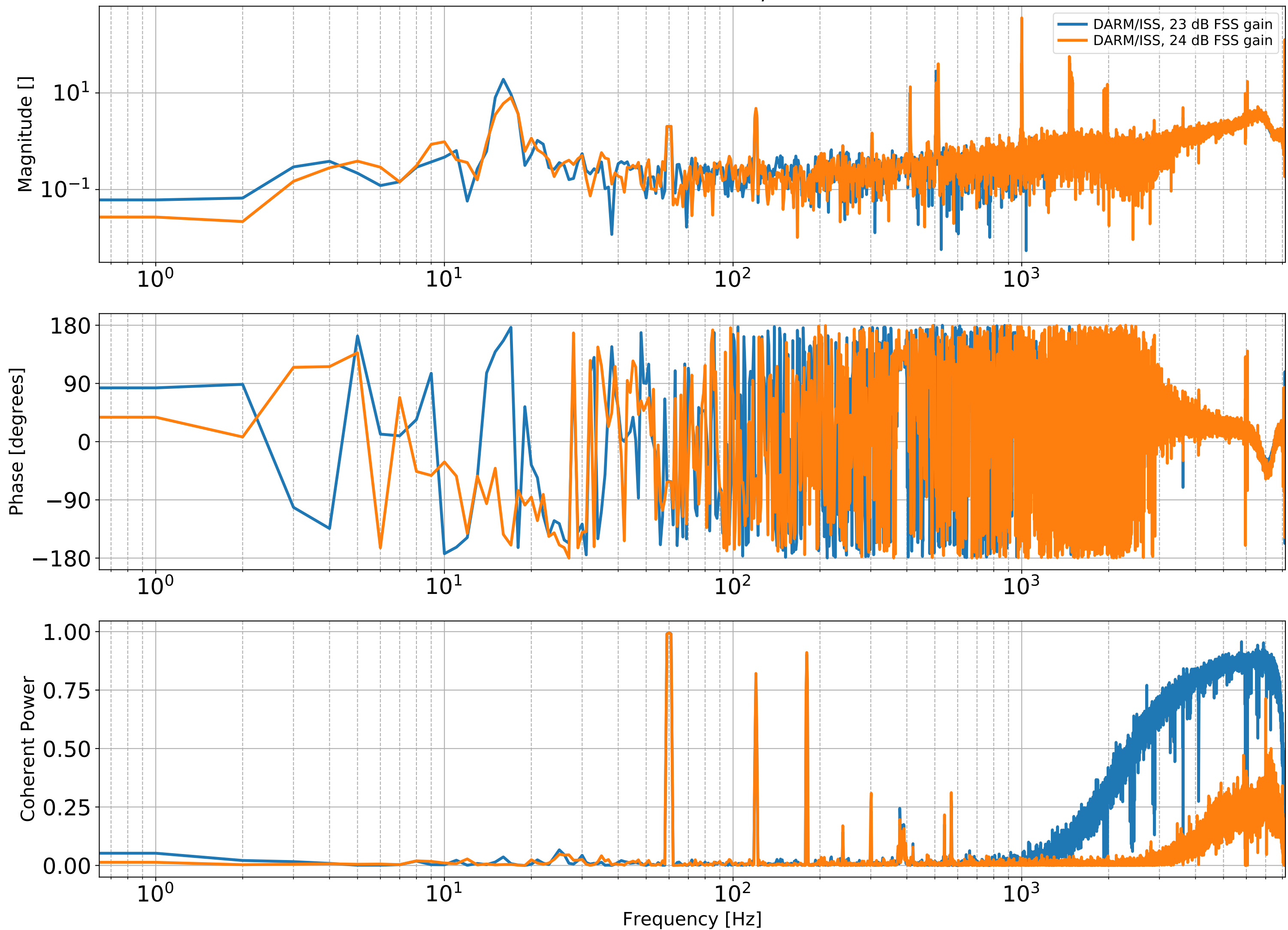
Uncalibrated DARM/ISS TF
