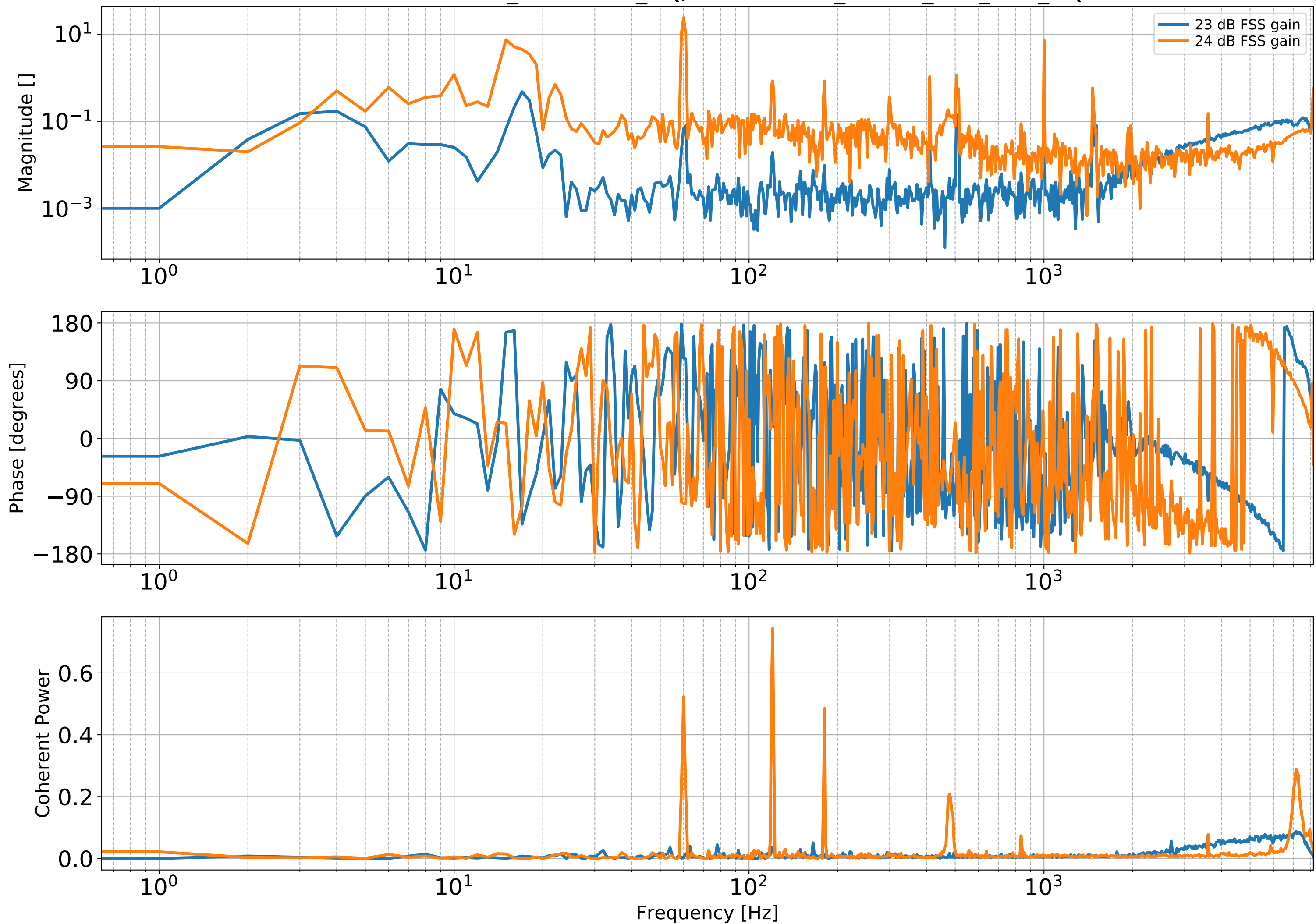
Uncalibrated DARM/CARM H1:CAL-DELTA_EXTERNAL_DQ/H1:LSC-REFL_SERVO_ERR_OUT_DQ
