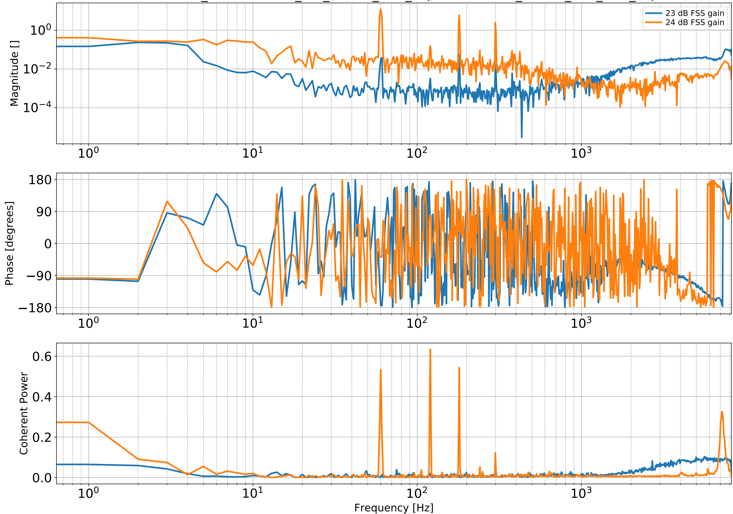
Uncalibrated ISS/CARM TF H1:PSL-ISS_SECONDLOOP_RIN_OUTER_OUT_DQ/H1:LSC-REFL_SERVO_ERR_OUT_DQ
