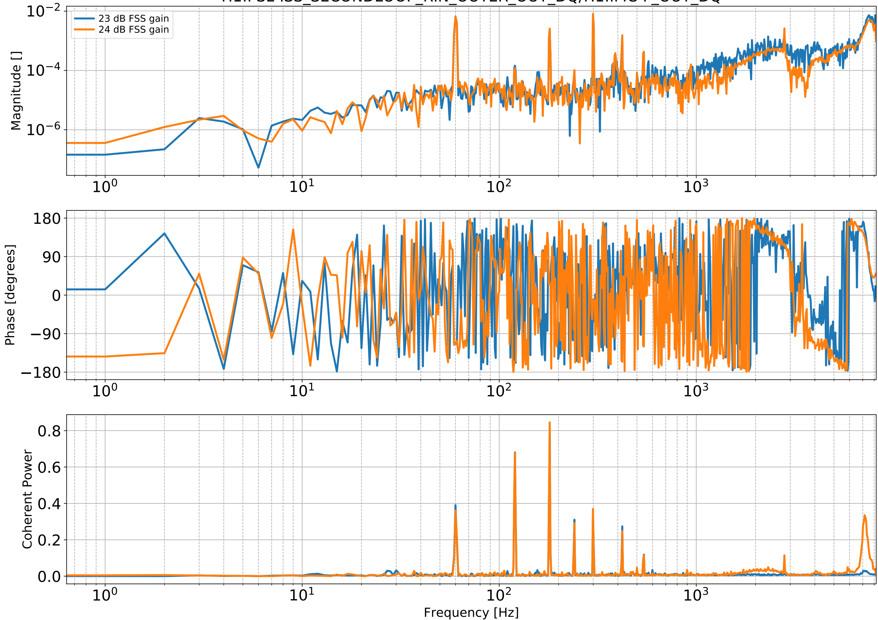
Uncalibrated ISS/IMC-F TF H1:PSL-ISS_SECONDLOOP_RIN_OUTER_OUT_DQ/H1:IMC-F_OUT_DQ
