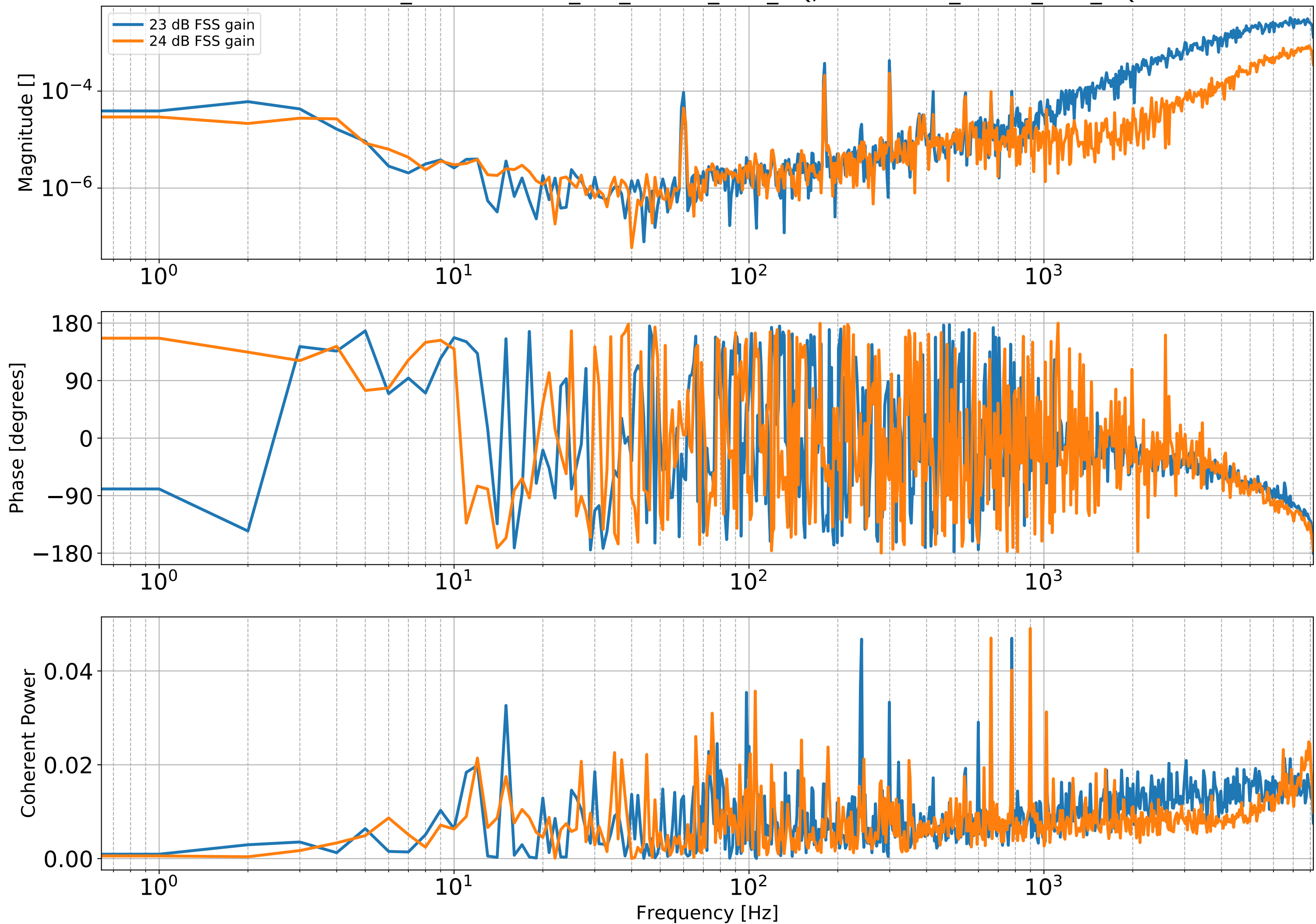
Uncalibrated ISS/FSS TF H1:PSL-ISS_SECONDLOOP_RIN_OUTER_OUT_DQ/H1:PSL-FSS_MIXER_OUT_DQ
