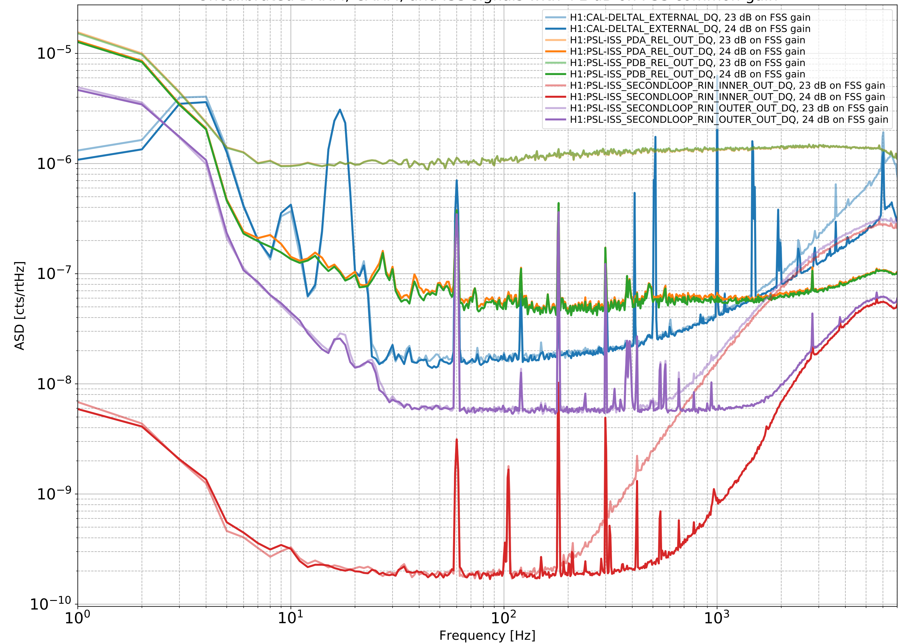
Uncalibrated DARM, CARM, and ISS signals with +1 dB on FSS common gain
