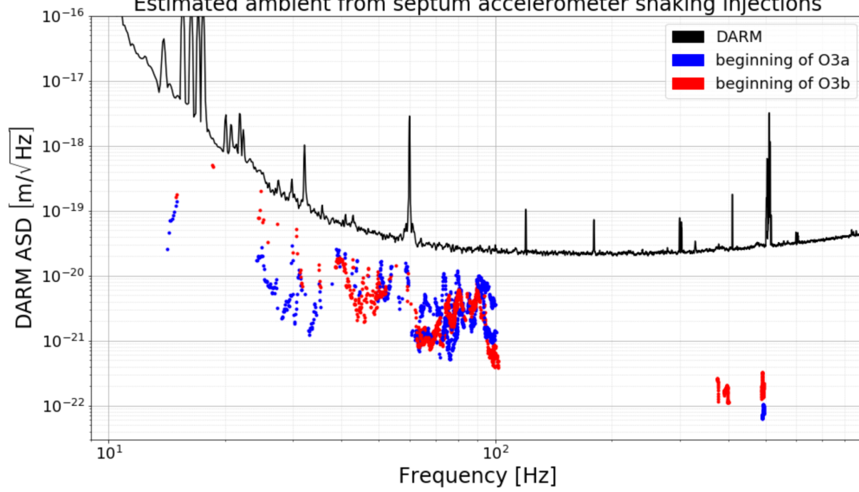
Septum accelerometer shaking injections
