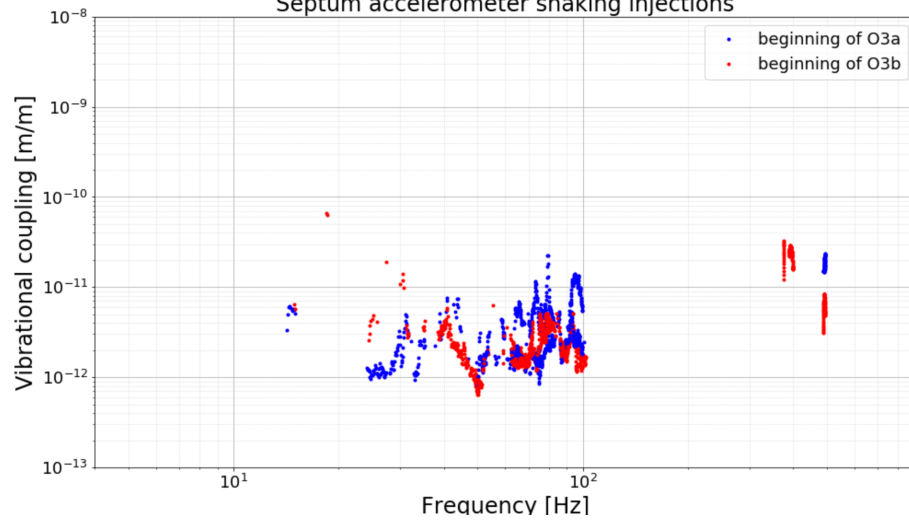
Septum accelerometer shaking injections
