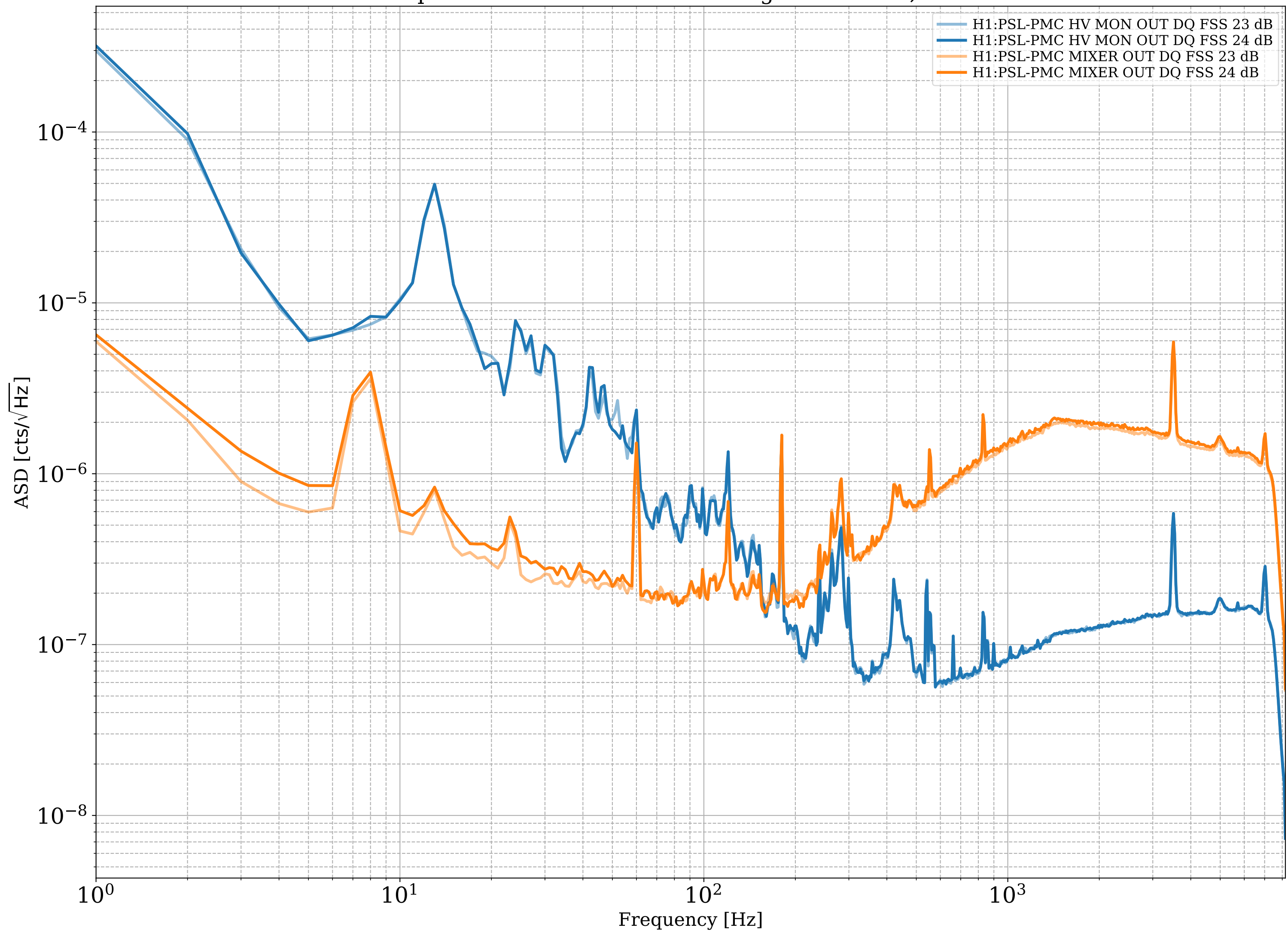
Spectra with 23 and 24 dB FSS gain - Nov 04, 2019
