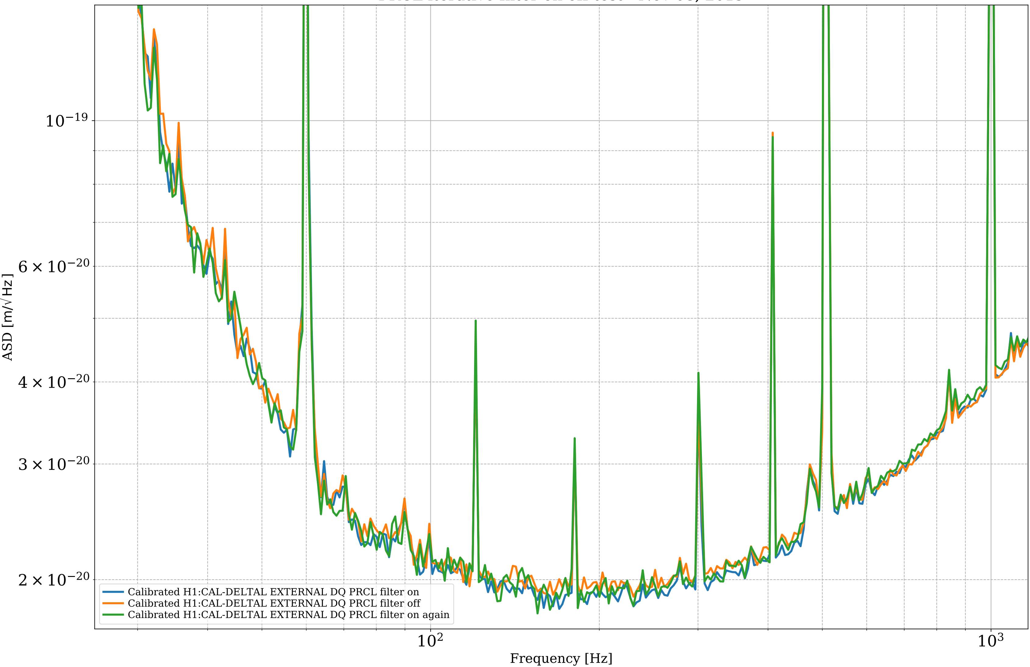
PRCL iterative filter on off test - Nov 08, 2019
