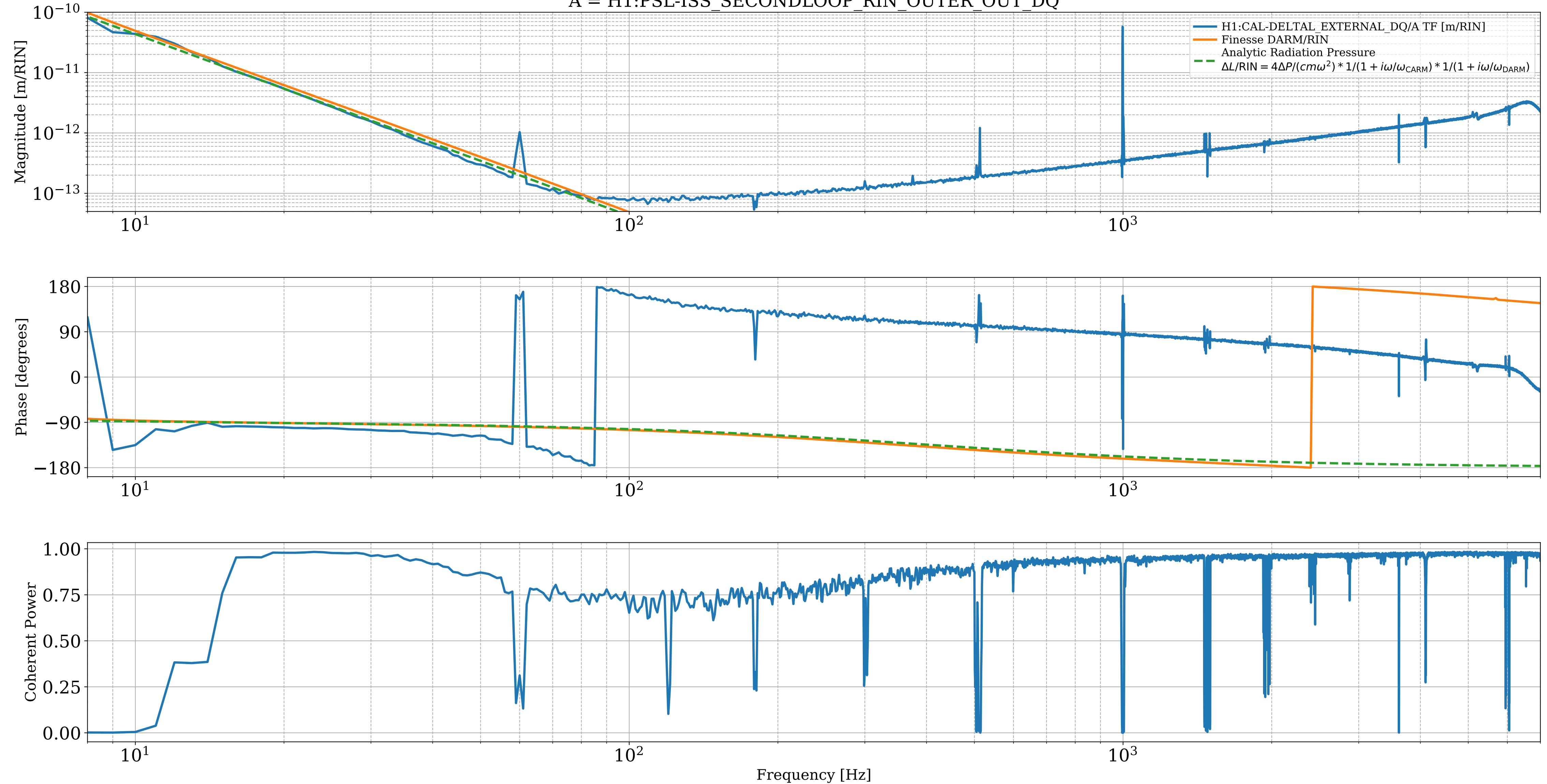
Measured vs Finesse vs Analytic DARM/Input RIN A = H1:PSL-ISS_SECONDLOOP_RIN_OUTER_OUT_DQ
