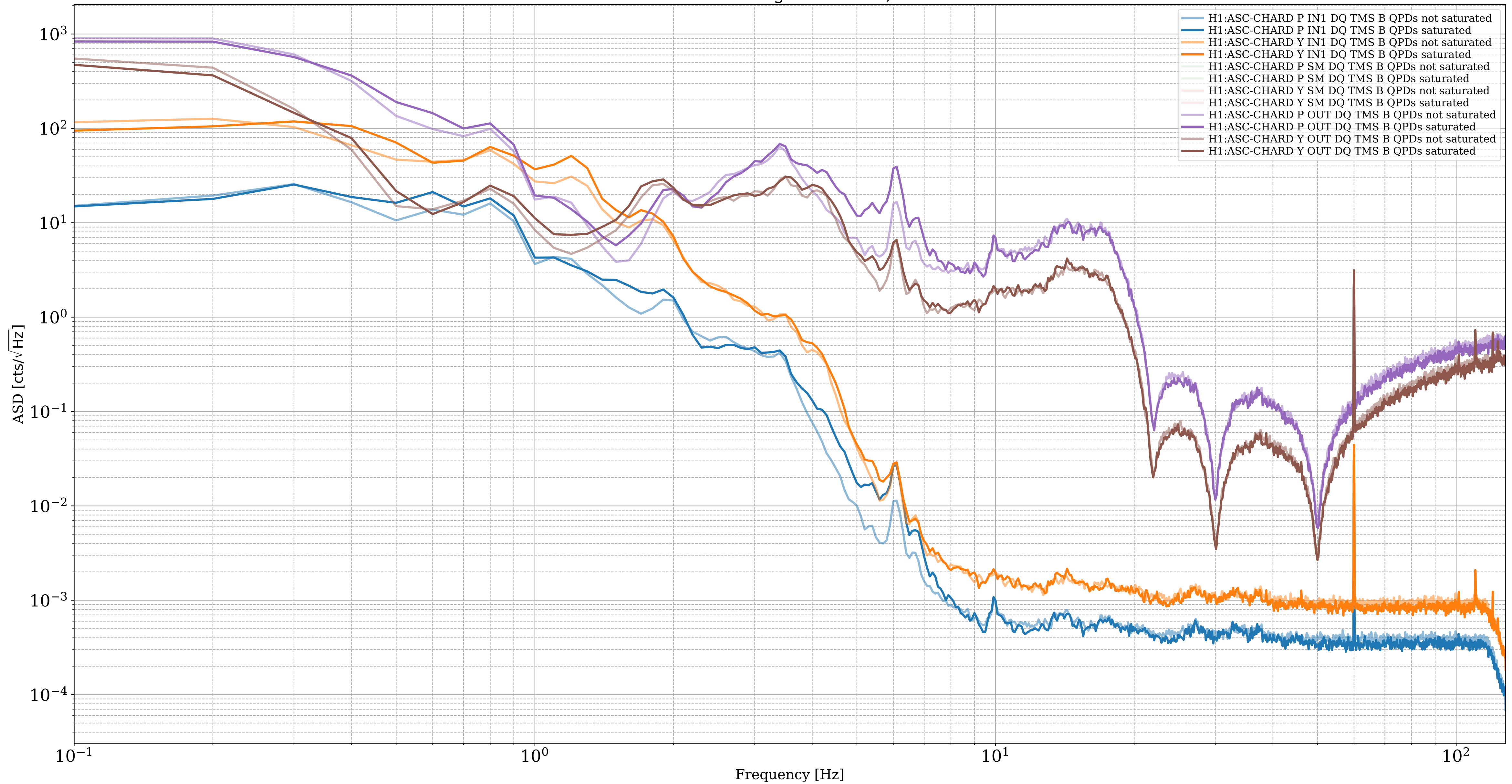
CHARD error signal - Nov 18, 2019
