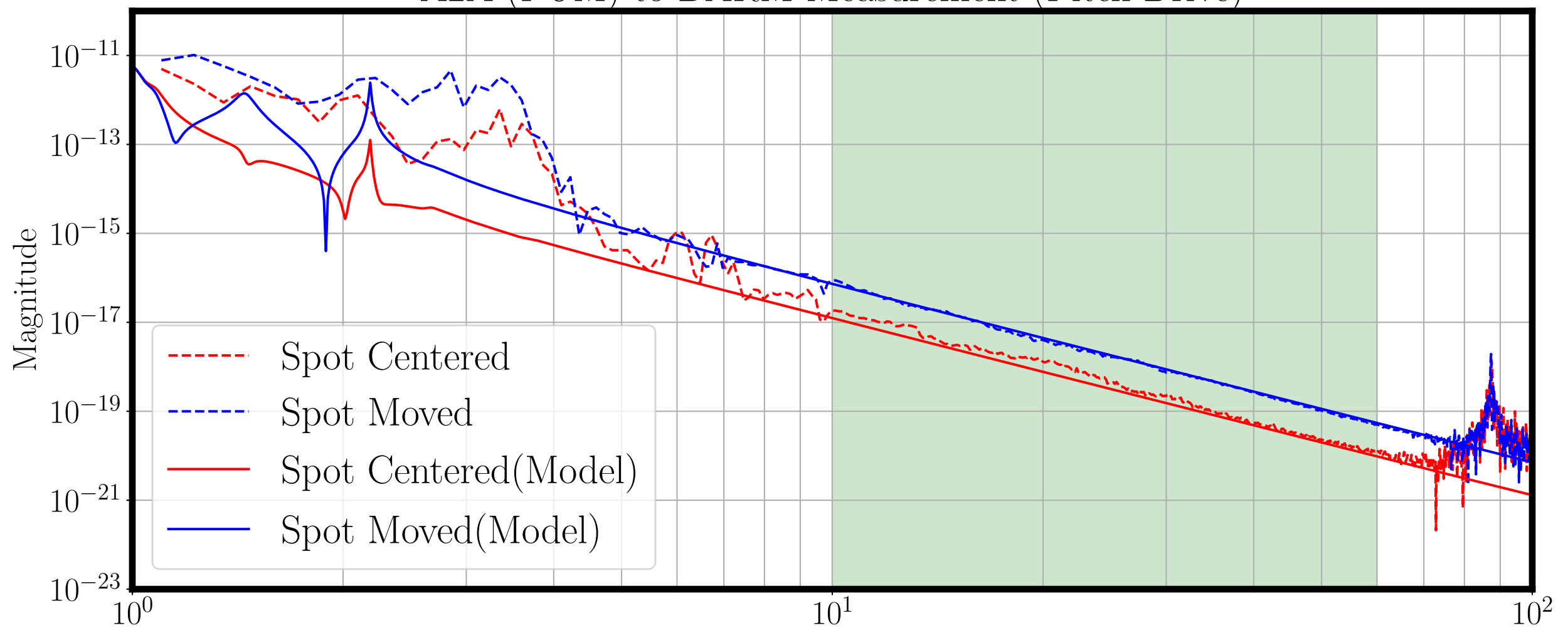
A2A (PUM) to DARM Measurement (Pitch Drive)
