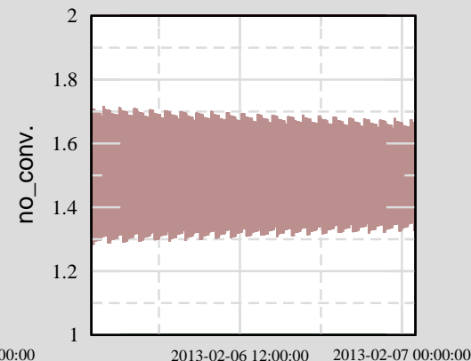
Ch 13: H0:PEM-LAB_DST1_MODE
