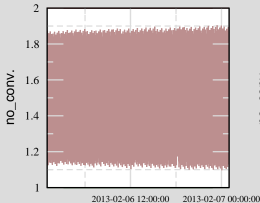
Ch 2: H0:PEM-LVEA_DST4_MODE
