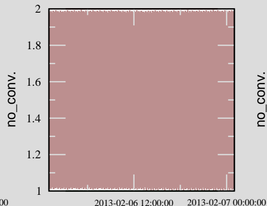
Ch 9: H0:PEM-LVEA_DST16_MODE
