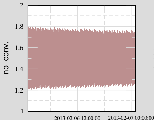
Ch 1: H0:PEM-LVEA_DST1_MODE
