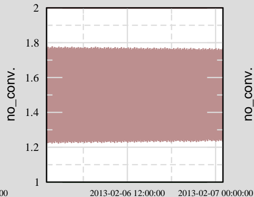
Ch 10: H0:PEM-EX_DST1_MODE
