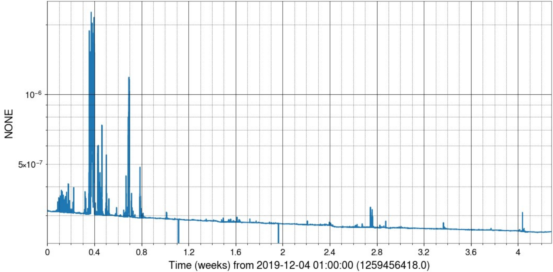
Time series: H0:VAC-LX_Y0_PT110_MOD1_PRESS_TORR.mean,m-trend Fs: (0.017 Hz), duration: 2592000.0
