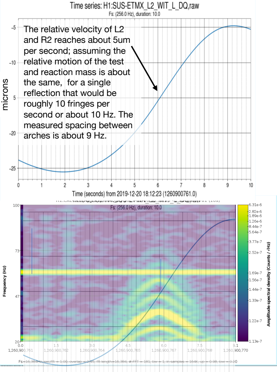
Fig. 1b. relative velocity of main and reaction chains can account for spacing between arches
