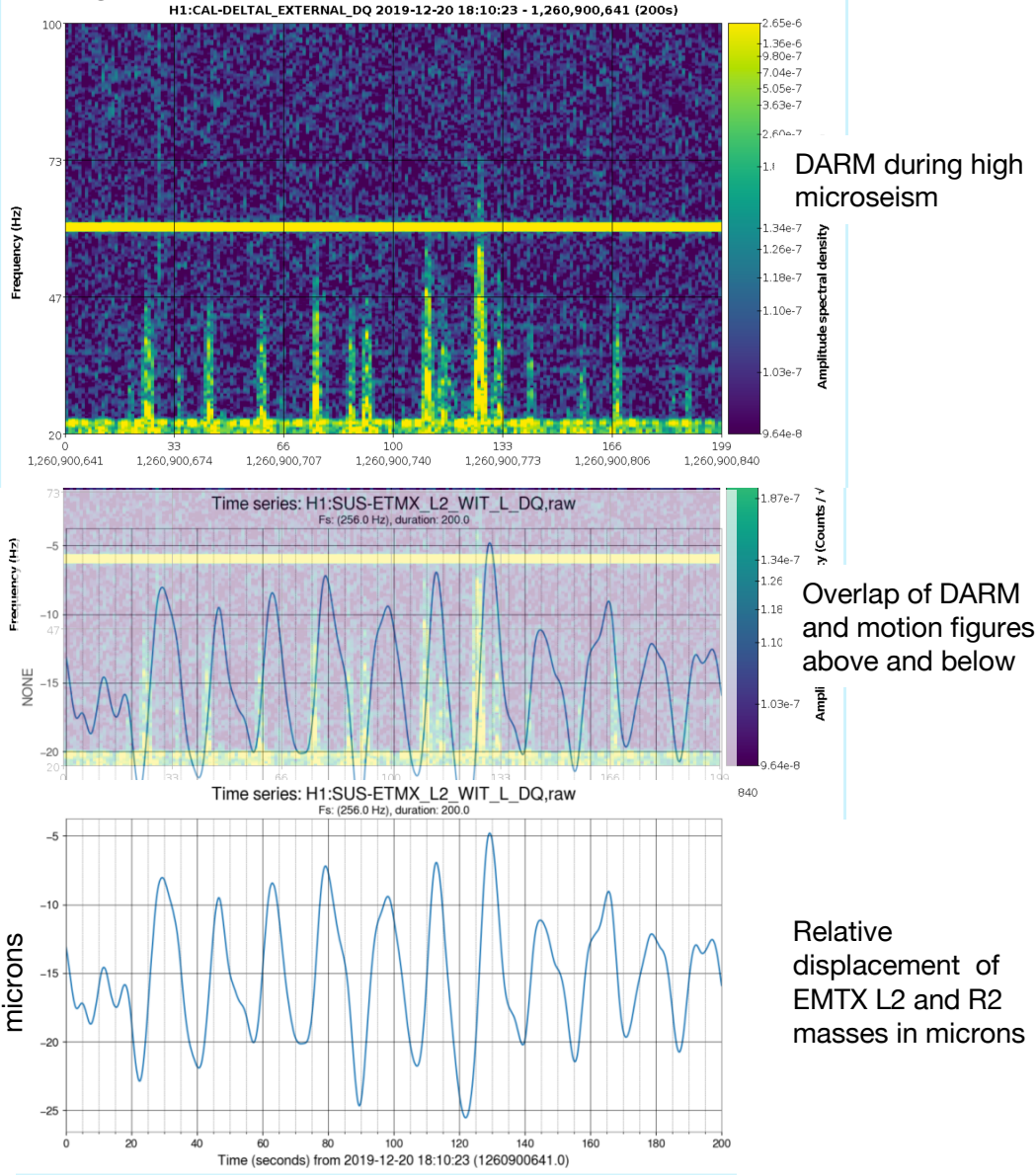
Fig. 1a. Scattering noise in LHO DARM correlates with rapid changes in ETMX L2 WIT L
