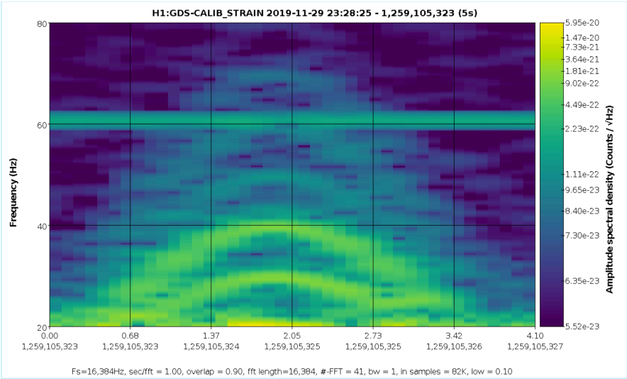
Figure 3. Each arch has an amplitude averaging 1/3 as large as the arch below it in frequency.
