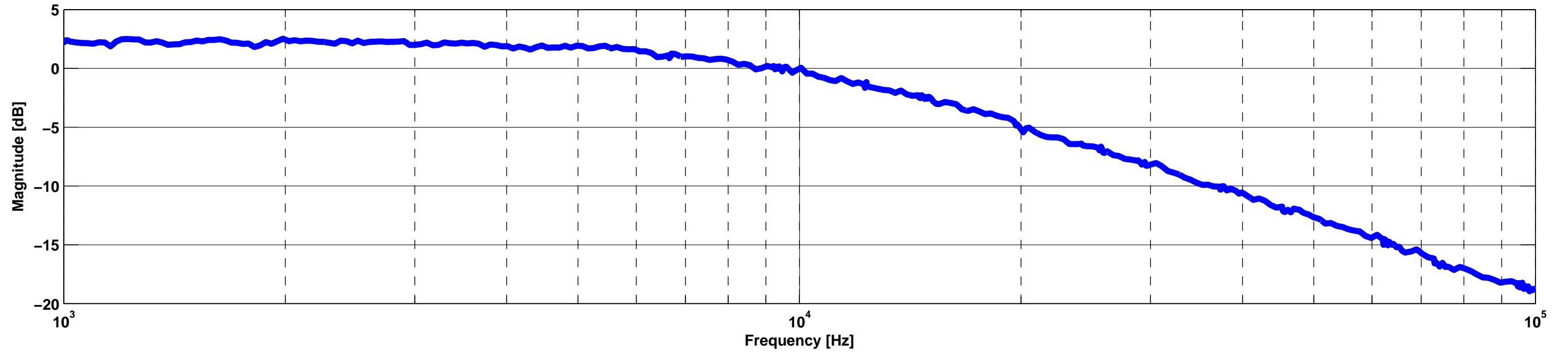
Initial TF from PSL PD to IOT2L PD in transmission, no PD calibration
