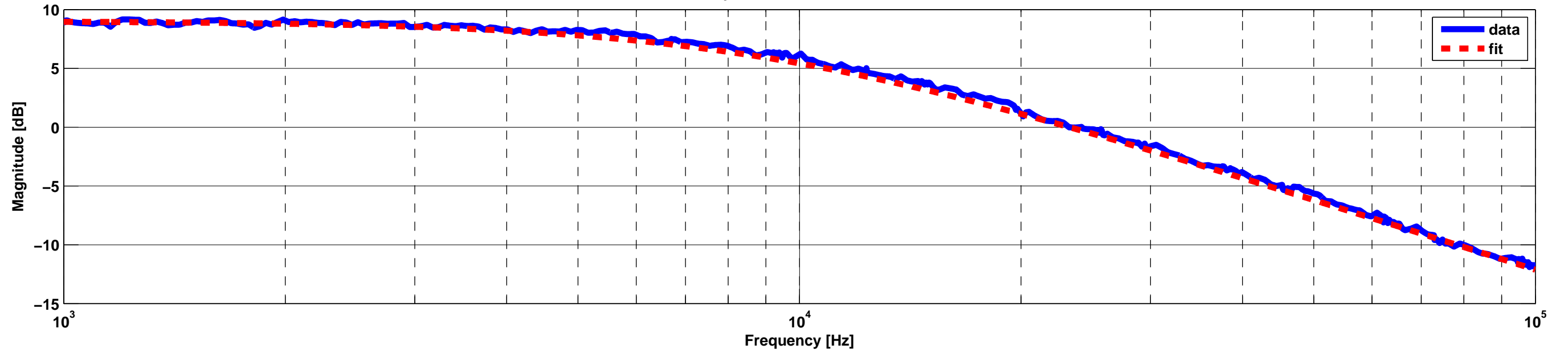
IMC pole measurement and fit
