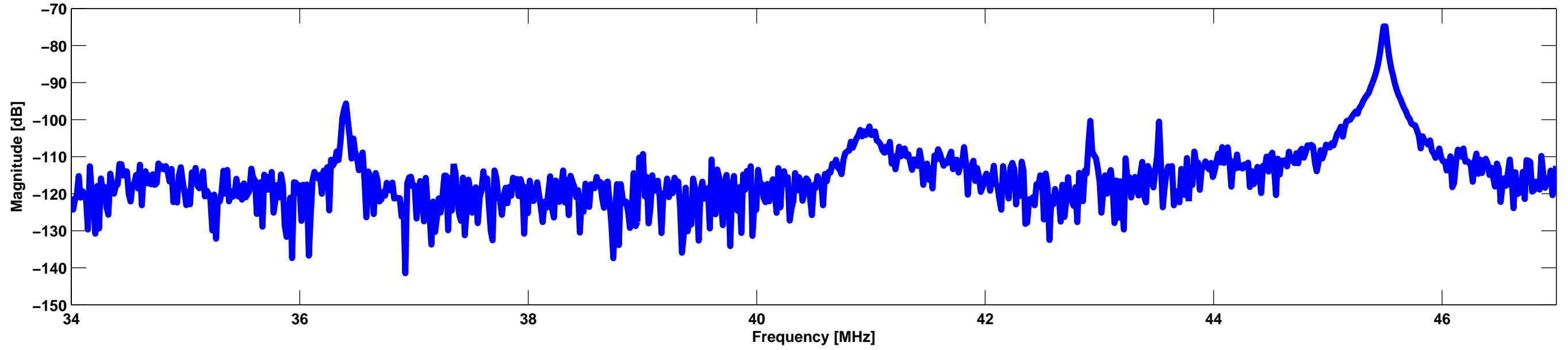
Sideband sweep full FSR
