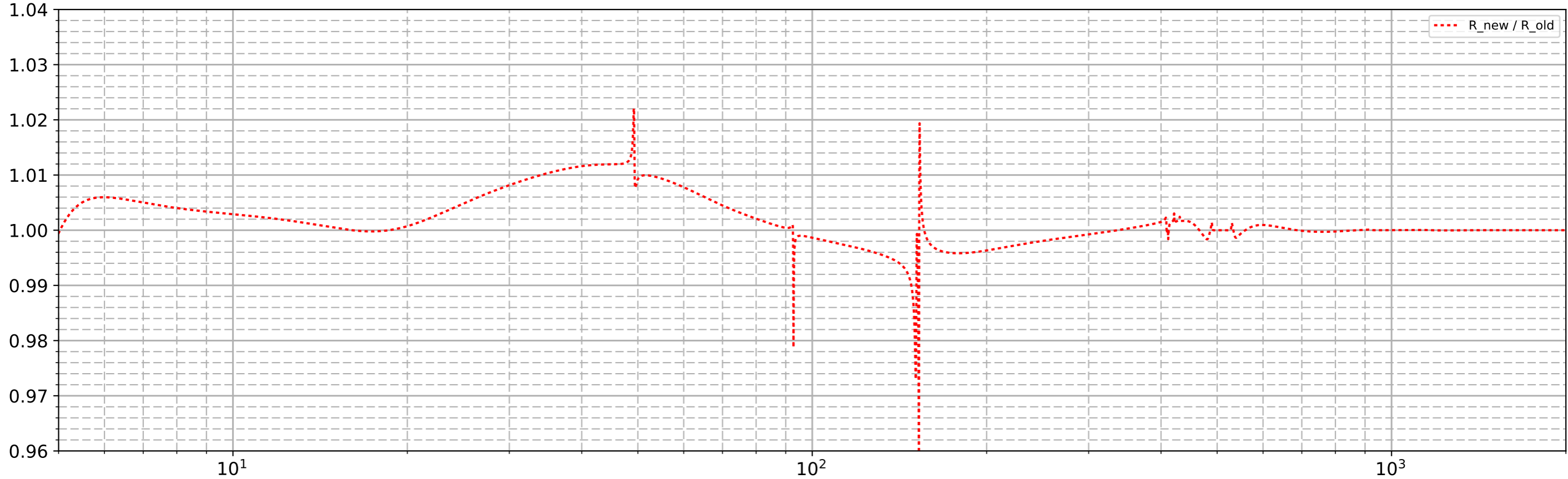
Ratio between: new R_foton (generated using foton filters for DELTAL) and old R_foton (generated using foton filters for DELTAL)
