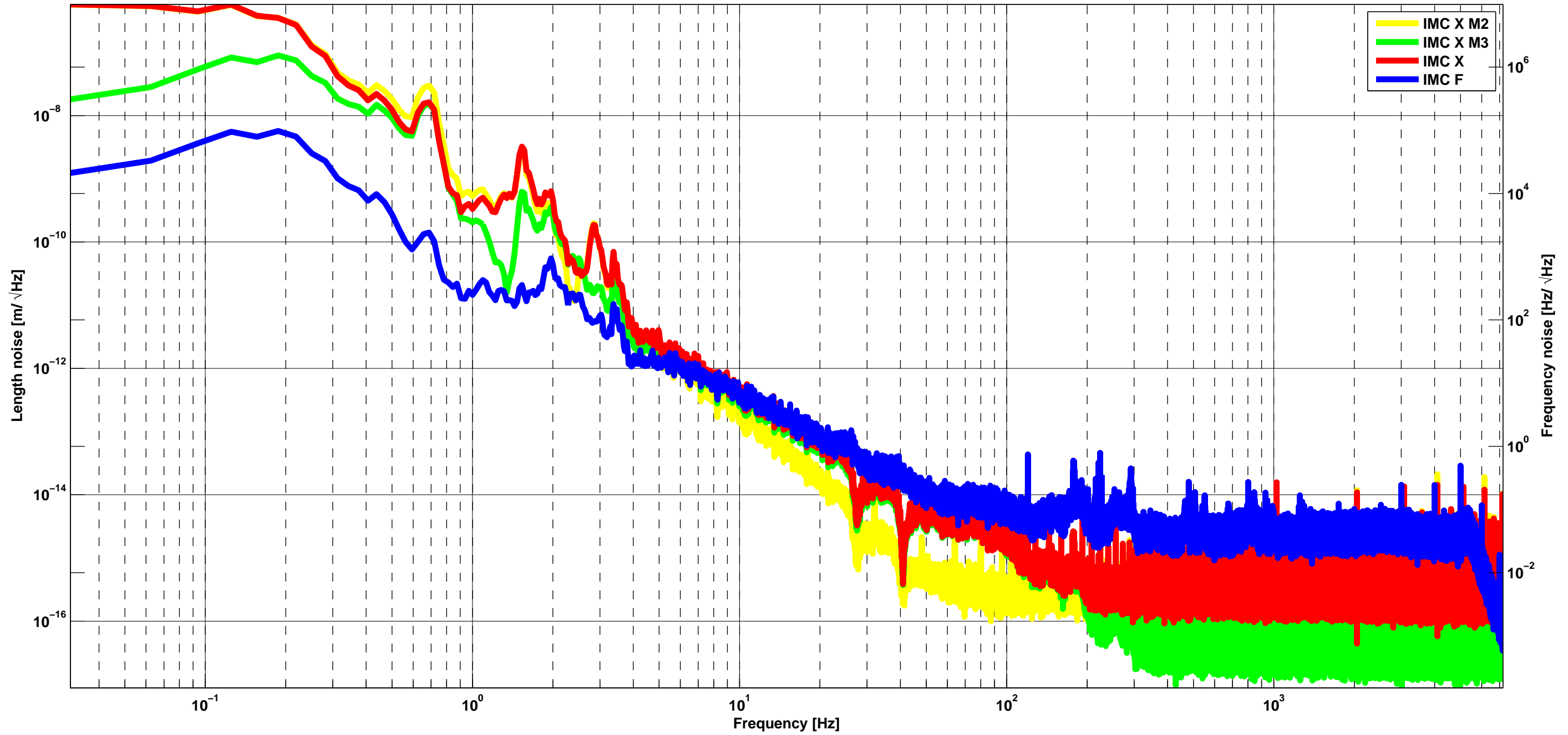
IMC length/frequency noise spectrum 2013/11/02
