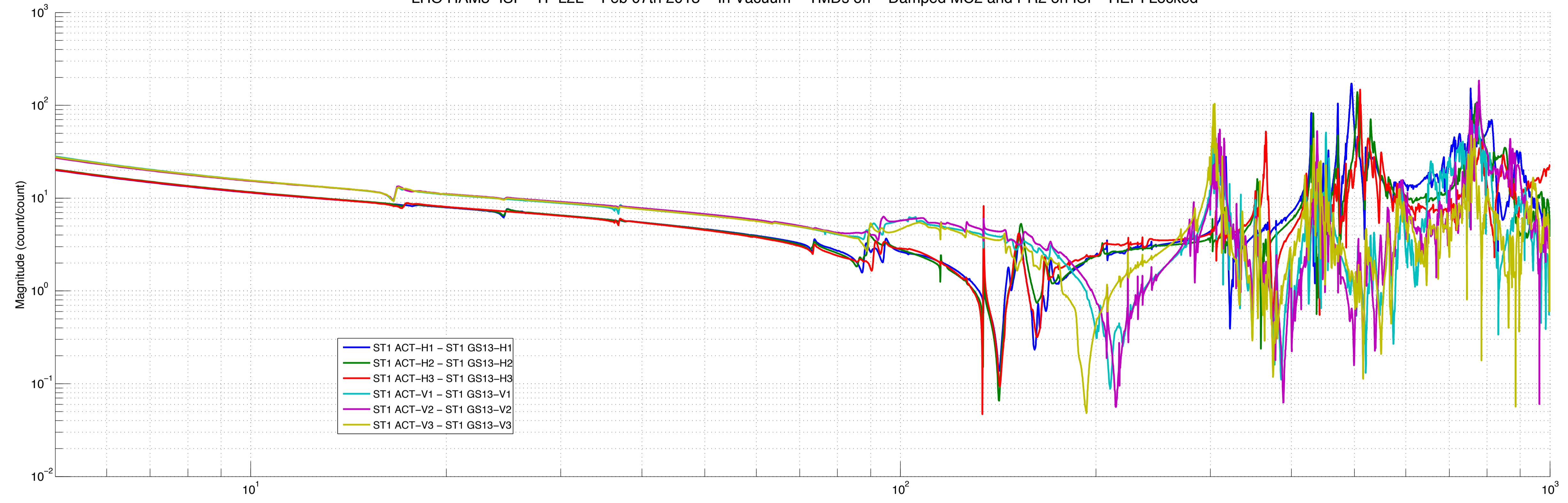
LHO HAM3-ISI - TF L2L - Feb 07th 2013 - In Vacuum - TMDs on - Damped MC2 and PR2 on ISI - HEPI Locked
