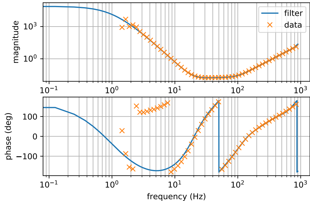
Inverse ETMXLLTransferFunction
