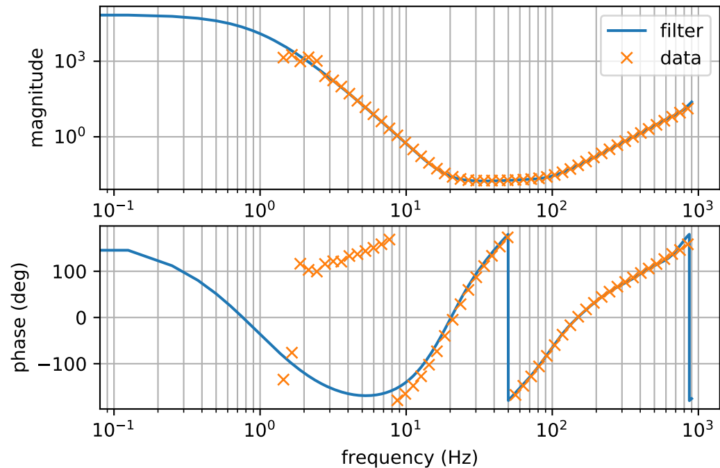
Inverse ETMYULTransferFunction
