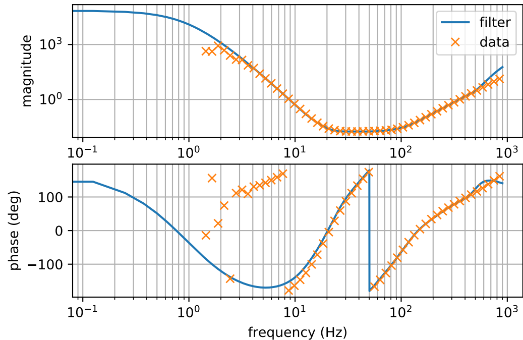
Inverse ITMXLRTransferFunction
