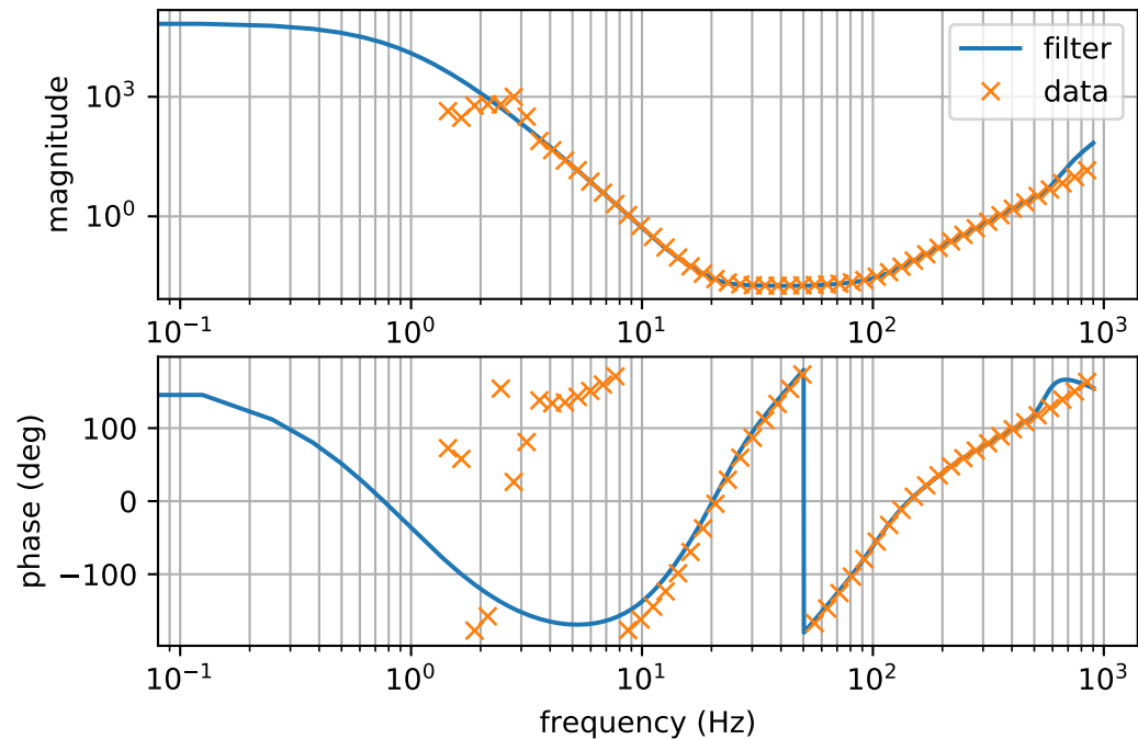
Inverse ITMXULTransferFunction
