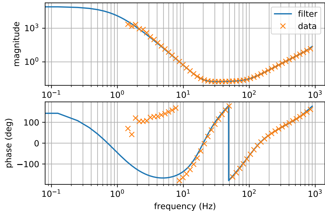
Inverse ITMYLRTransferFunction
