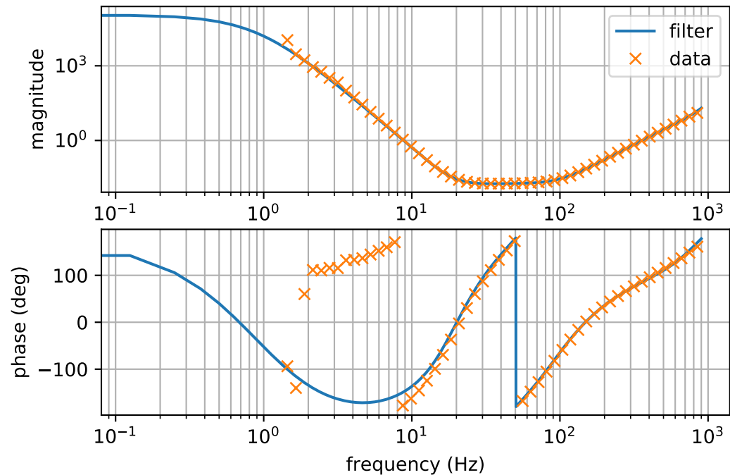
Inverse ETMYLRTransferFunction
