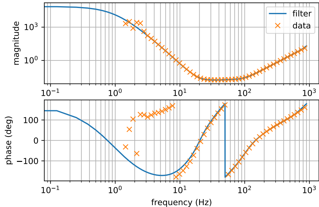
Inverse ETMXULTransferFunction
