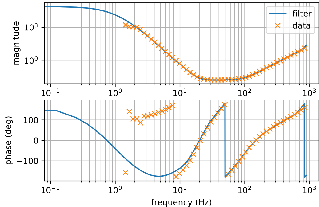
Inverse ITMYULTransferFunction
