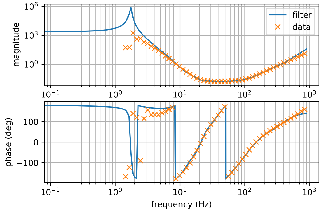
Inverse ITMXURTransferFunction
