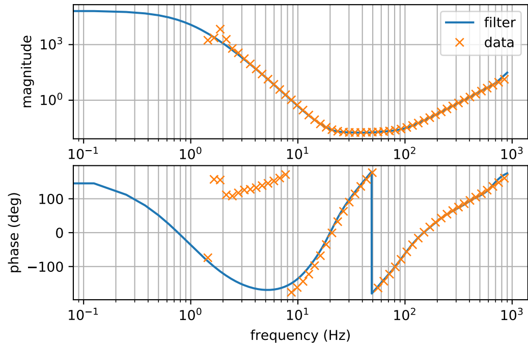
Inverse ETMXLRTransferFunction
