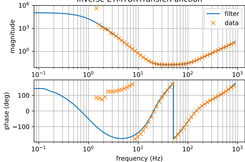
Inverse ETMYURTransferFunction
