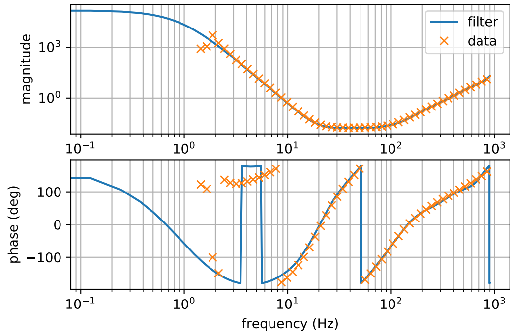
Inverse ETMYLLTransferFunction
