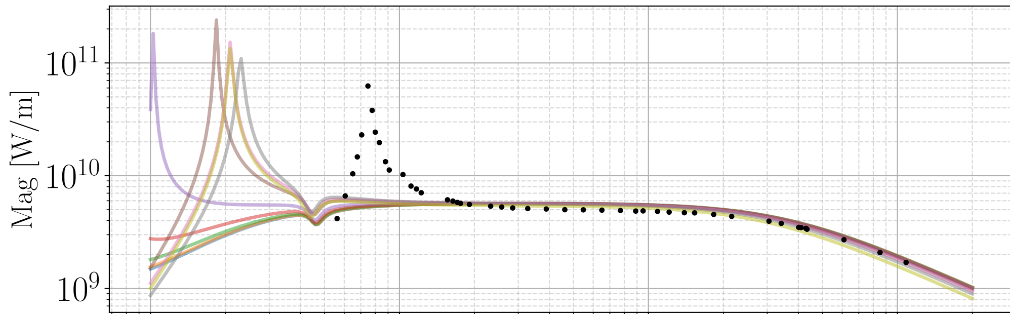
DARM TF with changes to \text{RoC}_{\text{SR3}} = 35.972841 \text{ m}
