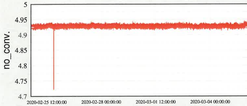
Ch 2: H0:VAC-MY_IP9_EI247_A_HV_KVOLTS
