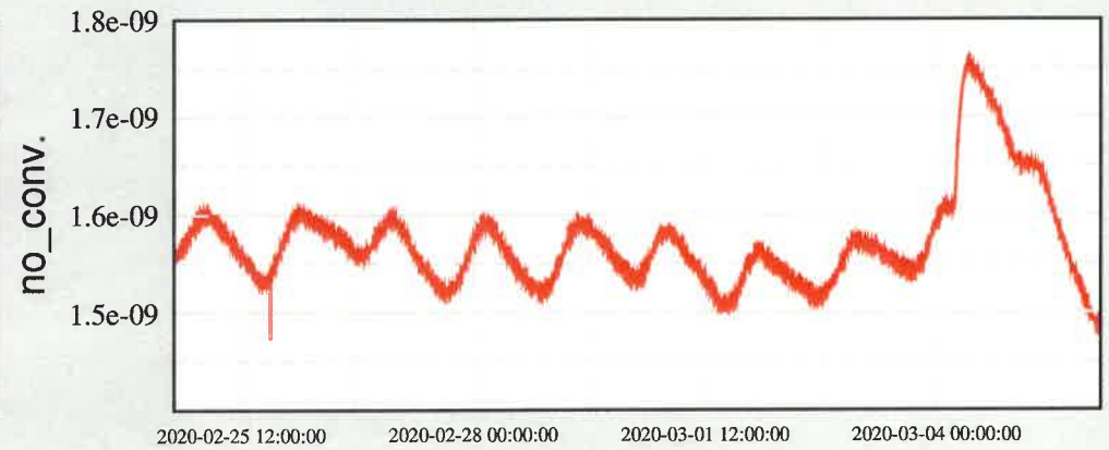
Ch 4: H0:VAC-MY_Y2_PT244B_PRESS_TORR
