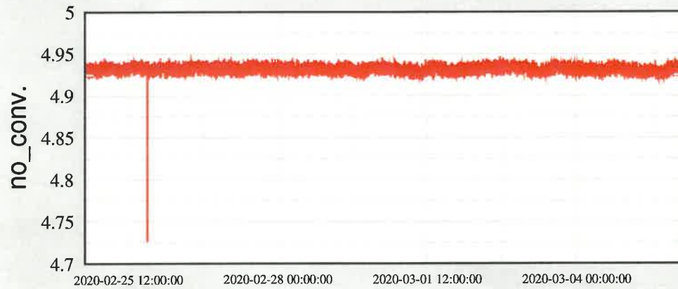
Ch 1: H0:VAC-MY_Y1_PT243B_PRESS_TORR
