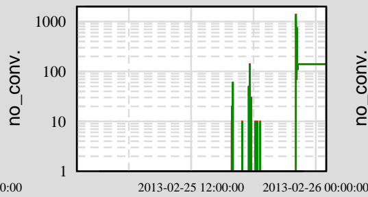
Ch 7: H0:PEM-LVEA_DST14_5
