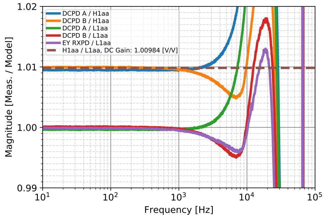
Anti-aliasing Chassis, Model vs. Measurement H1 O3B
