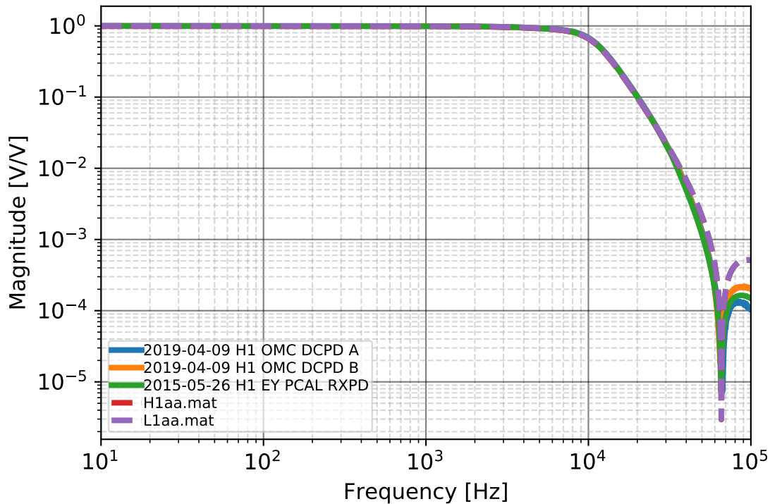
Anti-aliasing Chassis, Model vs. Measurement H1 O3B
