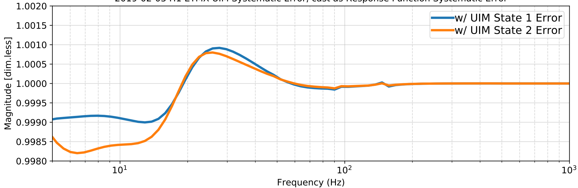
2019-02-03 H1 ETMX UIM Systematic Error, cast as Response Function Systematic Error
