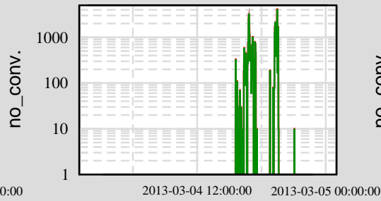
Ch 7: H0:PEM-LVEA_DST14_5
