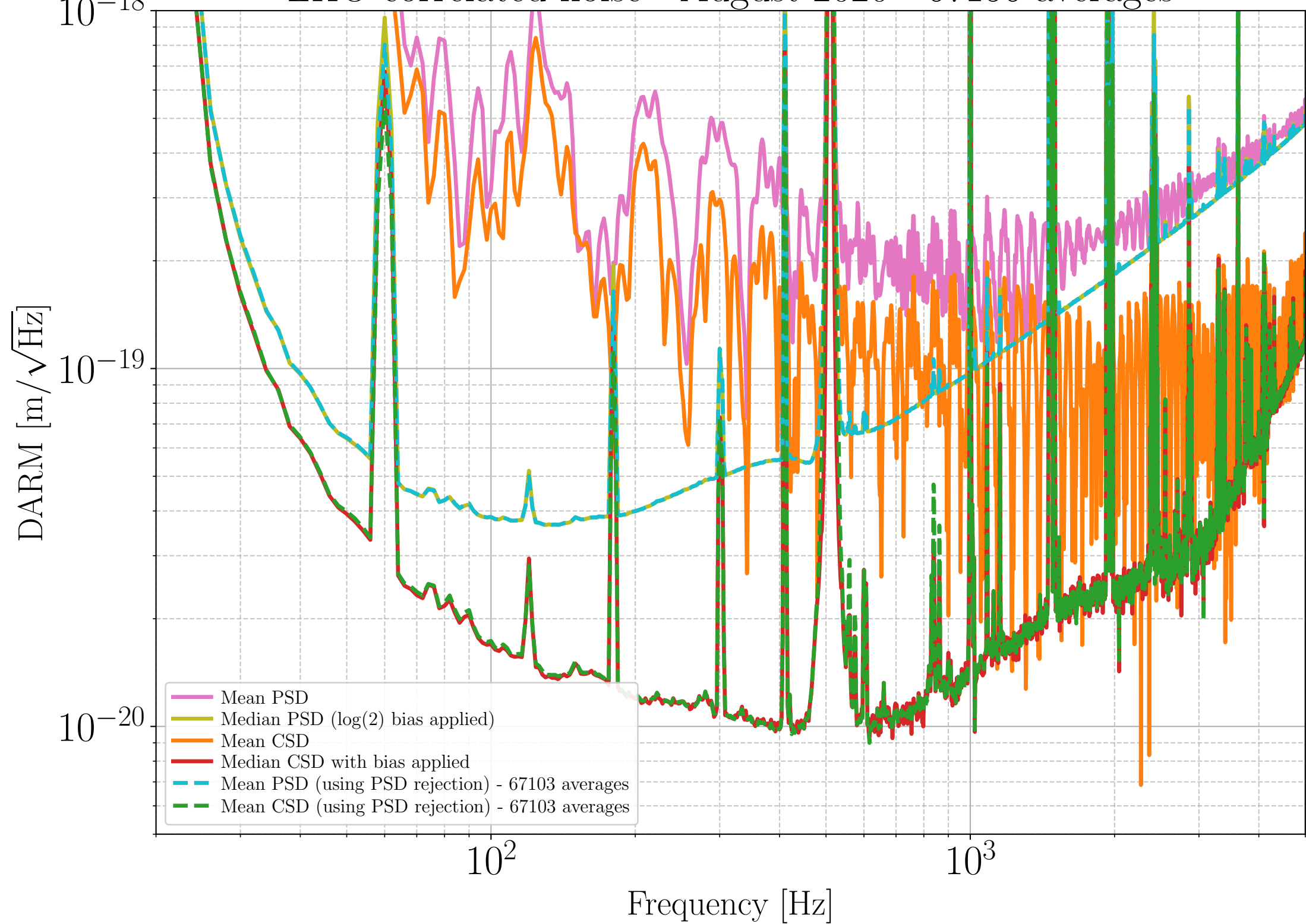
LHO correlated noise - August 2020 - 67156 averages
